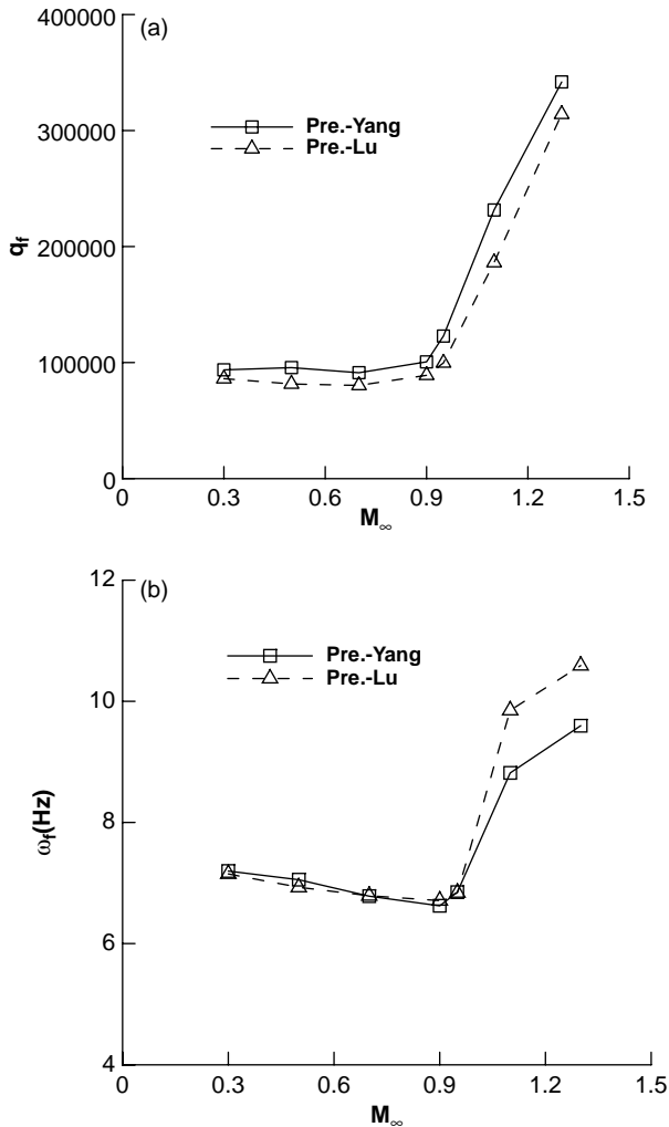
Figure 6. (a) Flutter dynamic pressure and (b) flutter frequency.
