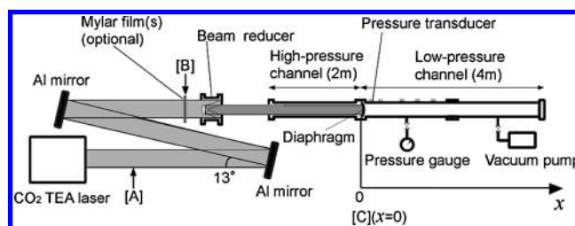
Fig. 1 Experimental setup.
