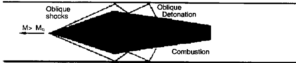
图10 Schematic of a ram accelerator for supersonic combustion propulsive mode
