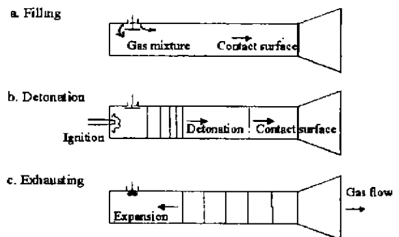
图 6 Thermodynamic cycle of Pulse Detonation Engines
