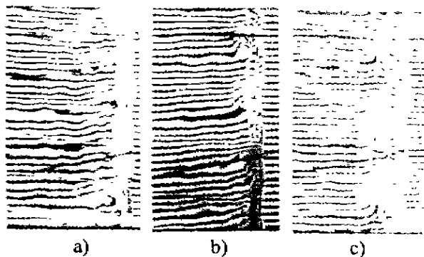
图 1 Interferogram of gaseous detonation structure of 2H_2 + O_2 + 0.92Xe at various initial pressures;
