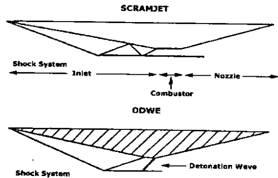
图 9 Schematic of shock structure for scramjet based on oblique detonation wave engines (ODWE)
