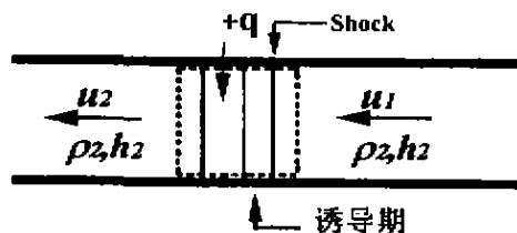
图 4 Schematic of detonation and control volume
