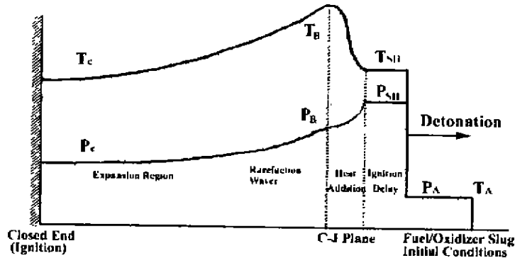
图 7 State variables distribution along detonation chamber
