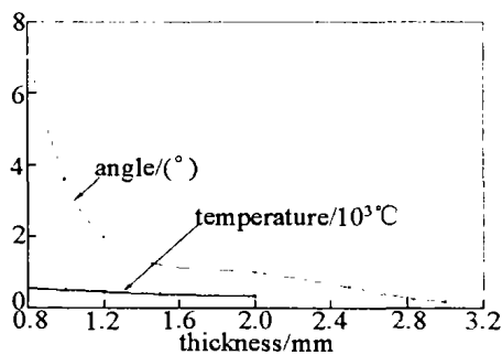
Fig. 9 The influence of sheet metal thickness on the bending angle v=16.67\text{mm/s} , P=500\text{W} , d=4\text{mm}
