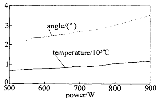
Fig. 6 The influence of laser output power on the bending angle v = 16.67 \text{ mm/s}, d = 4 \text{ mm}, s = 1.5 \text{ mm}
