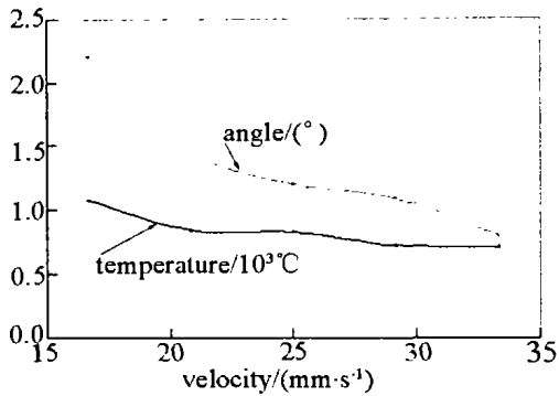
Fig. 7 The influence of laser beam scan velocity on the bending angle P=900\text{W} , d=4\text{mm} , s=2\text{mm}
