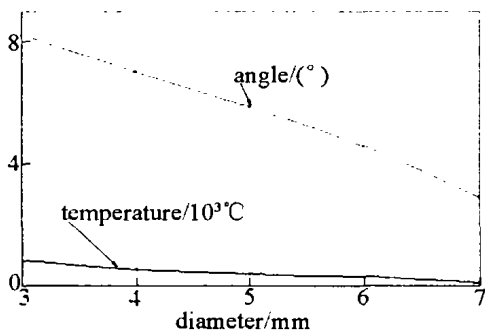
Fig. 8 The influence of laser beam diameter on the bending angle v=16.67\text{mm/s} , P=500\text{W} , s=0.8\text{mm}
