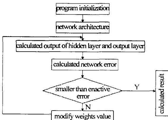
Fig. 2 Learn program flow diagram of BP network
