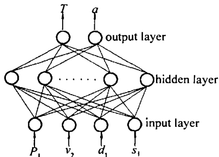
Fig. 1 The general architecture of BP network predicting bending angle
