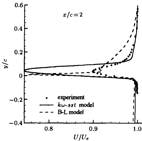
(b) 尾迹区速度剖面比较 (b) Comparison of velocity profiles
