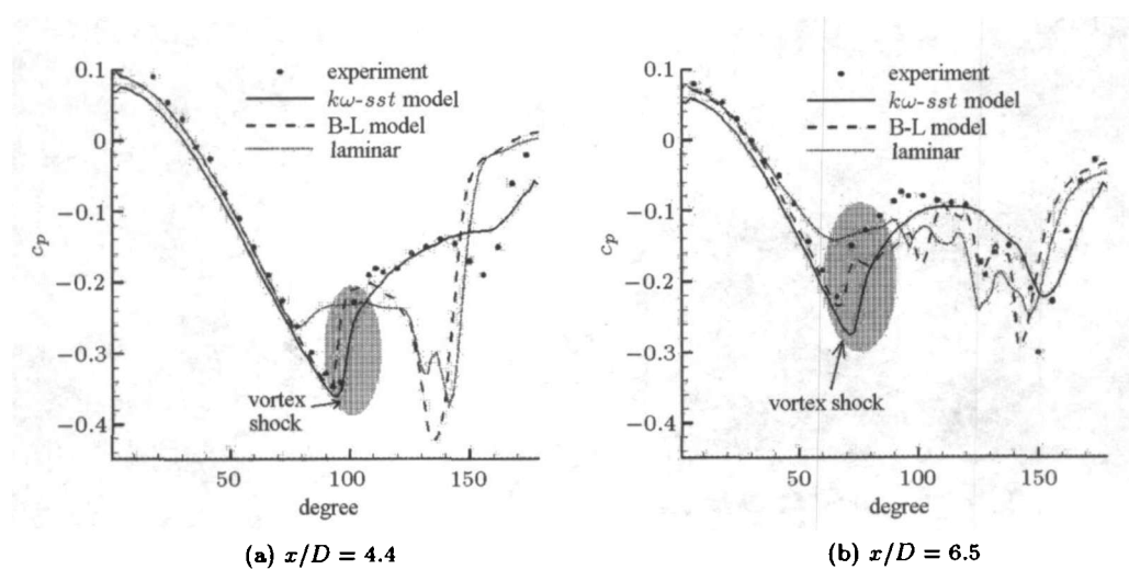
Fig.13 Surface circumferential pressure distribution (Case 3)
