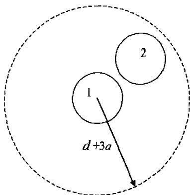
Fig. 1 The simulation model of the two hard spheres in an optical trap
