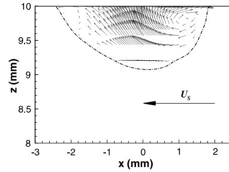
Fig. 7. Computed velocity vector field on the vertical symmetrical plane ( y = 0 ). T_0 = 14,000 K, U_0 = 400 m s ^{-1} , U_s = 2 mm s ^{-1} and d\sigma/dT = -5.0 \times 10^{-4} kg s ^{-2} K ^{-1} .
