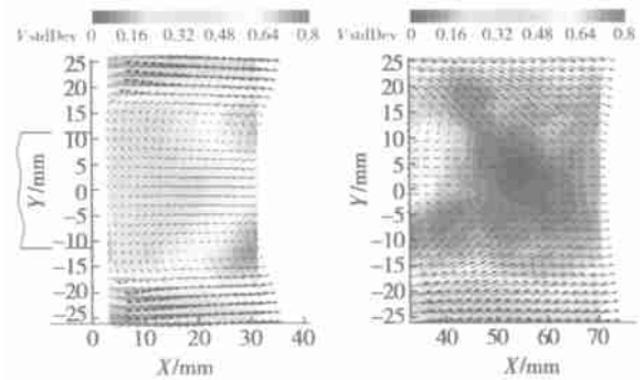
Fig. 5 Mean flow field behind the novel flameholder ( \theta = 180^\circ ) V_m = 10\text{m/s} V_j = 20\text{m/s}
