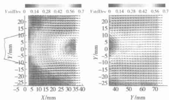
(b) Velocity vector and contour of transverse fluctuating velocity
