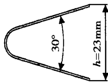
Fig. 2 Sketch of the V-gutter flameholder
