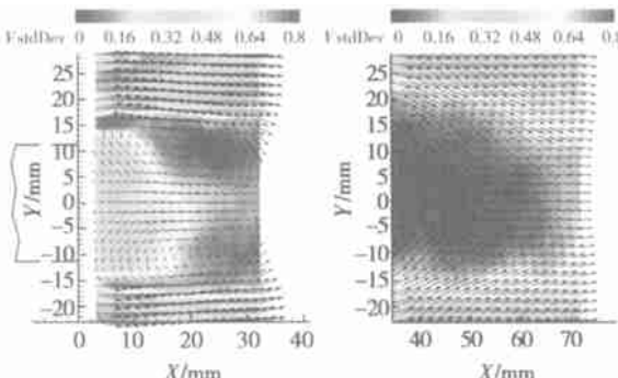
Fig. 9 Mean flow field behind the novel flameholder ( \alpha = 120^\circ ) V_m = 10\text{m/s} V_j = 20\text{m/s}
