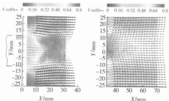
Fig. 6 Mean flow field behind the novel flameholder ( \alpha = 180^\circ ) V_m = 20\text{m/s} V_j = 10\text{m/s}
