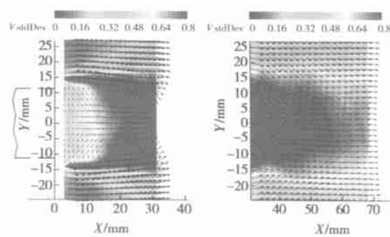
Fig. 8 Mean flow field behind the novel flameholder ( \alpha = 90^\circ ) V_m = 10\text{m/s} V_j = 20\text{m/s}
