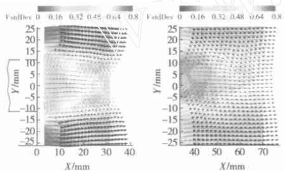
Fig. 7 Mean flow field behind the novel flameholder ( \alpha = 180^\circ ) V_m = 20\text{m/s} V_j = 20\text{m/s}
