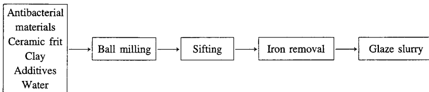
Fig. 1 Preparation of glaze slurry
