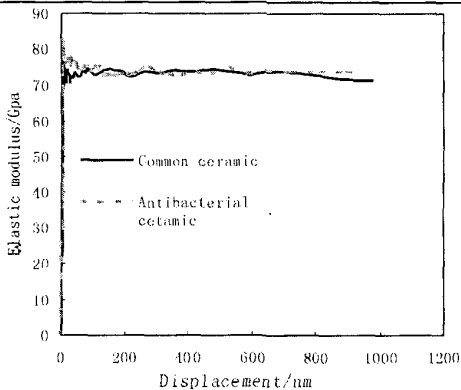
Fig. 5 Elastic modulus vs. displacement curves
