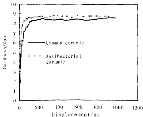
Fig. 6 Hardness vs. displacement curves
