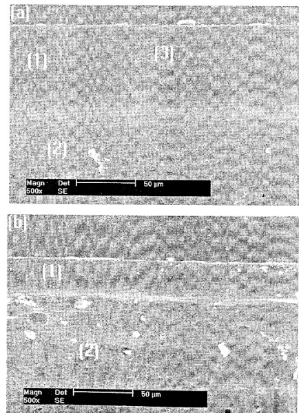
Fig. 2 SEM fracture surface appearance with and without antibacterial materials
