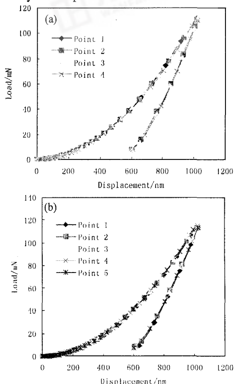
Fig. 4 Load vs. displacement curves on sample points (a) Common ceramic; (b) Antibacterial ceramic
