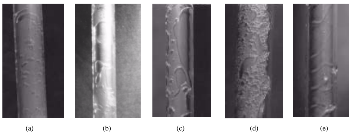
Fig.4 Flow patterns in narrow gap annular gap: (a) isolated bubble regime; (b) slug flow; (c) churn flow; (d) coalesced bubble regime; (e) annular flow.
