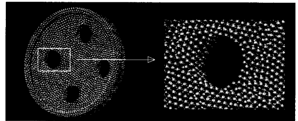
Figure 15: A local view of sphere packing around a hole
