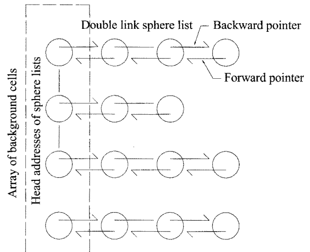
Figure 5: Data structure of the background system
