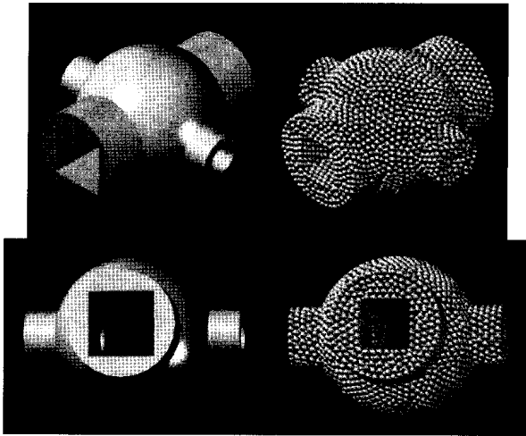
Figure 12: Axle sleeve and its final packing of internal spheres
