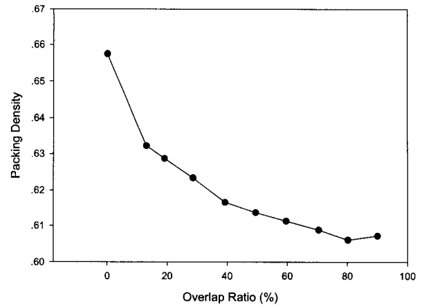
Figure 2: Packing density vs. overlap rate
