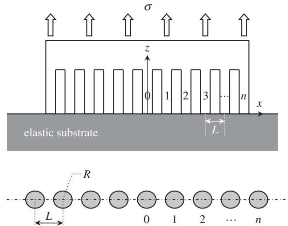
Figure 5. Schematic of a large number of identical rigid and cylindrical fibrils which are in perfect contact with an elastic substrate. Each fibril has radius R \leq R_{cr} , and the interface tractions between each fibril and substrate are assumed to be homogeneous theoretical interface strength at pull-off to find the constraints on the number of fibrils.
