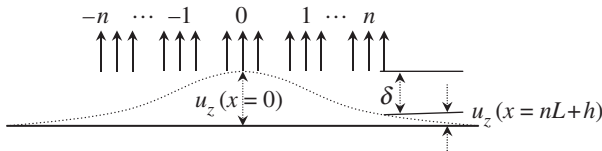
Figure 3. Schematic of the deformation of an elastic half-plane under uniformly distributing tractions. The maximum separation is denoted by \delta .
