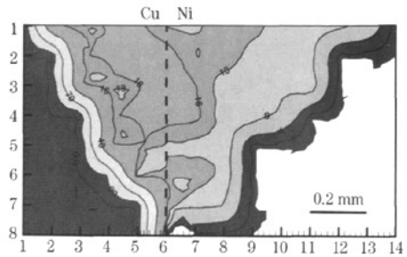
图4 焊缝区铜元素含量分布图(虚线为焊缝中心) Fig. 4 Composition map of Cu over whole of weld pool (dotted line indicates centerline of weld)
