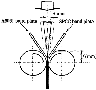
图2 激光压辊焊接过程图 Fig. 2 Schematic diagram of laser roll welding
