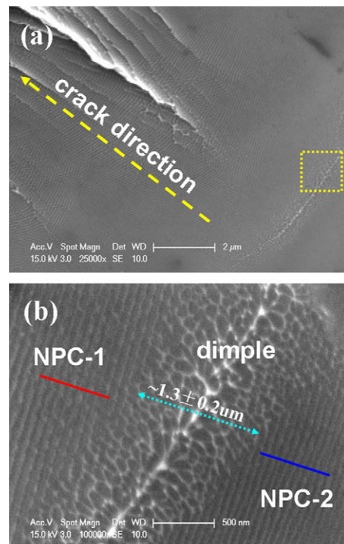
Figure 2. (a) NPC on the dynamic mode I fracture surface of Vit 1 BMG; (b) dimple formation in the NPC-predominated region marked in (a).
