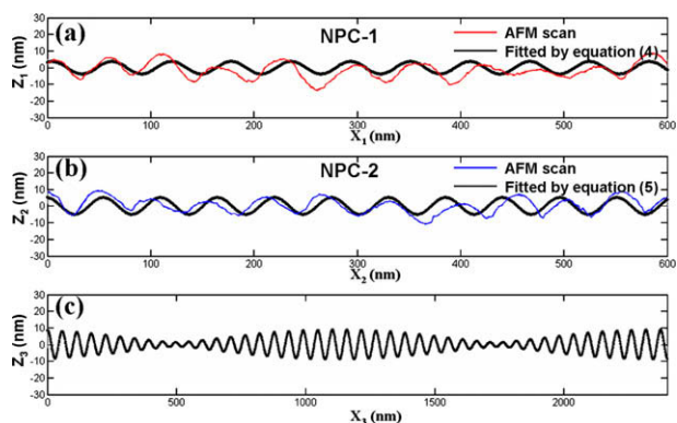
Figure 3. (a) AFM profile of NPC-1 marked in Figure 2(b), fitted by Eq. (4); (b) AFM profile of NPC-2 marked in Figure 2(b), fitted by Eq. (5); (c) superposition of Eqs. (4) and (5) showing a well-known beat phenomenon.
