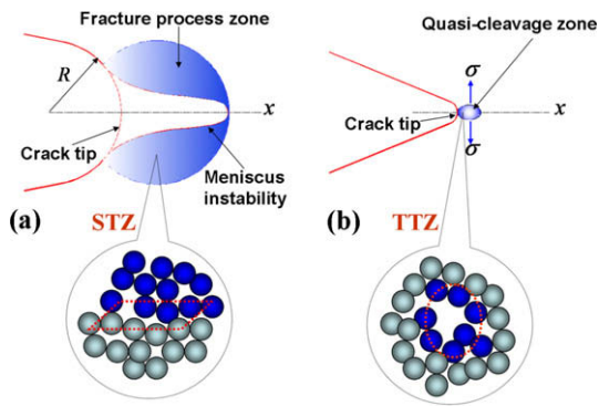
Figure 1. Schematic diagram of the ductile-to-brittle transition mechanism of metallic glasses during fracture. (a) If the curvature radius of the crack tip is greater than the critical wavelength of the meniscus instability, a ductile fracture will occur in the fracture process zone, where atomic clusters move via STZs, as shown in the inset; (b) in the opposite case, local quasi-cleavage fracture through TTZs (see the inset) is possible ahead to the sharp crack tip.
