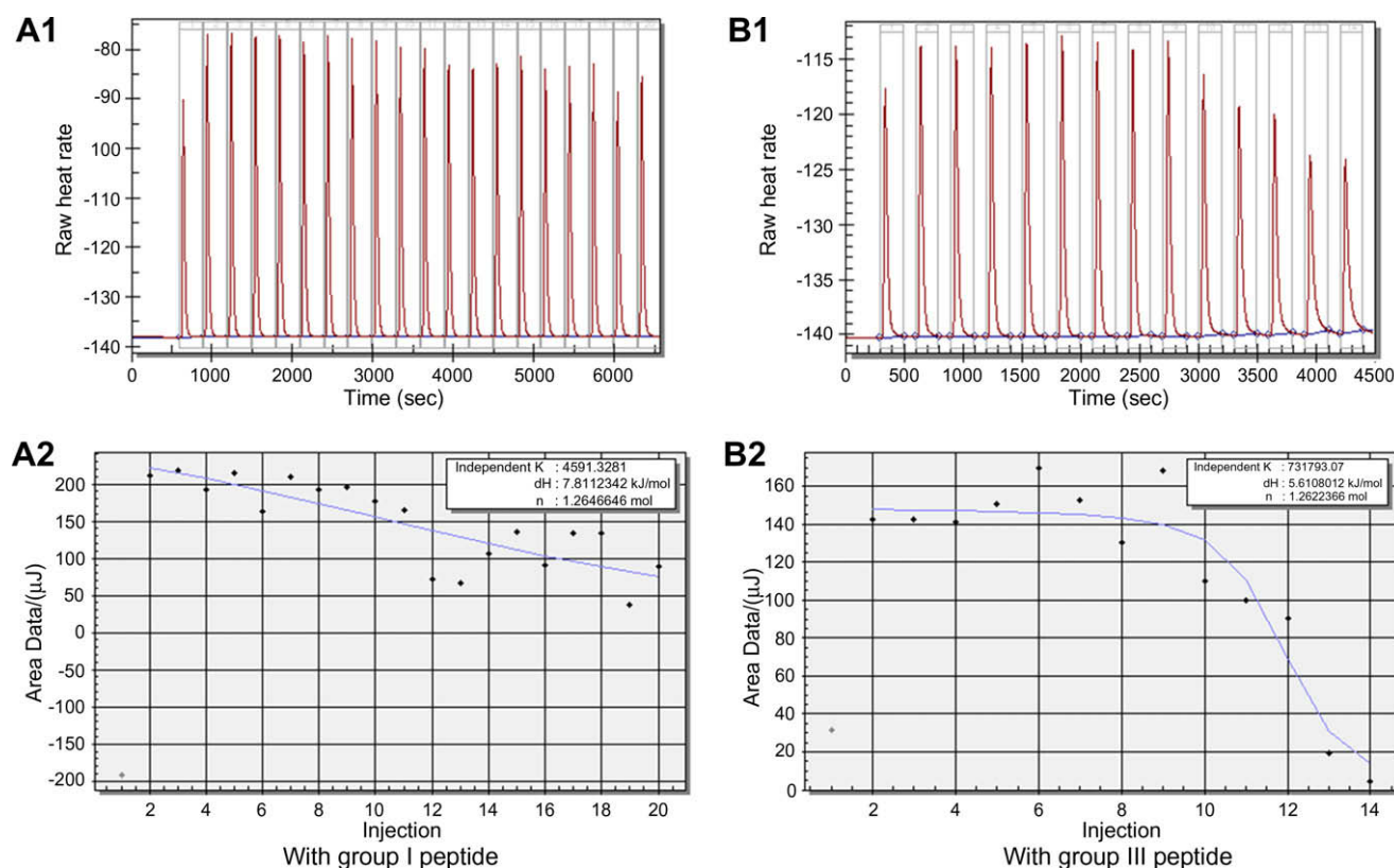
Fig. 3. Results of heat changes and data fitting made by the isothermal titration calorimeter NANOITC 2C and the software NaNoAnalysis, respectively. The binding assays of artificial protein 1 with group-I and group-III peptides are shown as examples. The binding constants can be calculated by K_D = 1/K . (A) The 500 \mu\text{M} artificial protein 1 was prepared in the sample cell. The 8 mM group-I peptide was injected into the cell with 5 \mu\text{l} per time, every 300 s. Data on heat changes are shown in (A1) and are fitted as reported in (A2). Data on the first injection were omitted because they are not accurate due to the initialization of the device. The results reported in (B1) and (B2) are of group-III peptide (5.3 mM) titrating into artificial protein 1 (250 \mu\text{M} ), using a similar approach.
