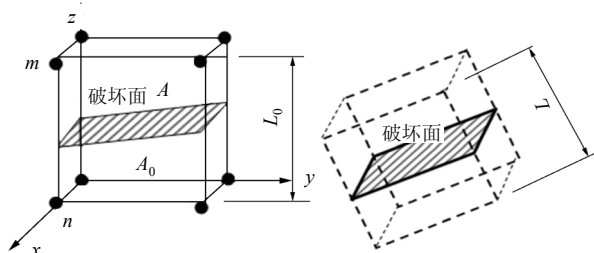
图9 破坏面切割块体示意图 Fig.9 Diagram of cutting block with failure interface
