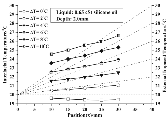
Fig. 2 The interfacial temperature profiles in 0.65 cSt silicone oil at different temperature differences (Dash line: external imposed temperature gradients)
