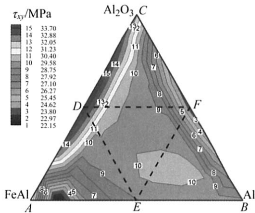
Fig.10 Distribution of maximal shear stress \tau_{xy} at Al/FeAl interface
