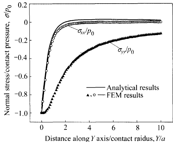
Fig.4 Analytical and FEM solutions for stresses along Y axis
