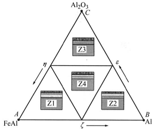
Fig.2 Zone division in triangle of normalized layer thickness
