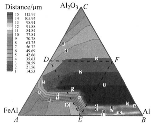
Fig.8 Distance of maximal \tau_{xy} from surface
