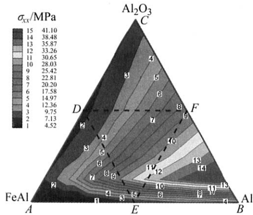
Fig.5 Distribution of maximal STS \sigma_{xx} in triangle
