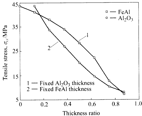
Fig.6 Effect of FeAl or Al_2O_3 layer on STS \sigma_{xx}
