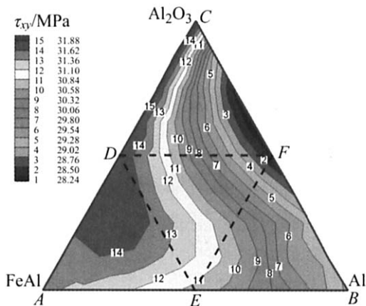
Fig.11 Distribution of maximal shear stress \tau_{xy} at FeAl/ Substrate interface
