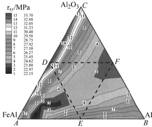
Fig.9 Distribution of maximal shear stress \tau_{xy} at Al_2O_3/Al interface
