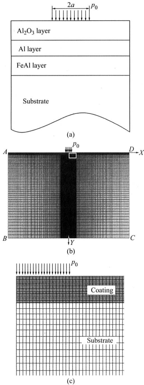
Fig.3 FEM model of HDA/PEO coating: (a) Uniform contact pressure; (b) FEM meshes; (c) Magnified image of local meshes
