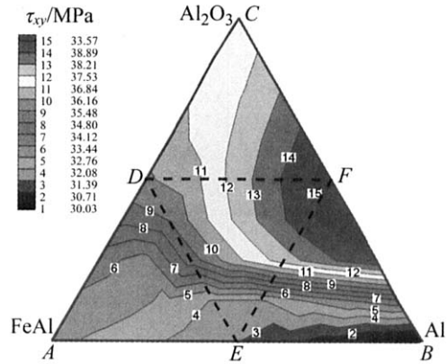
Fig.7 Distribution of maximal shear stress \tau_{xy}
