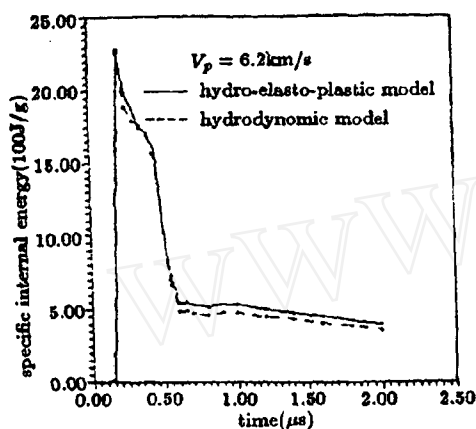
图 3 (0, 1.5) 处比内能随时间的变化曲线 Fig.3 Specific internal energy at the center in the mid-section of the shield
