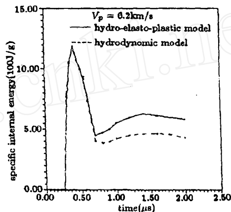
图 4 (2.5, 1.5) 处比内能随时间的变化曲线 Fig.4 Specific internal energy at off-axis point ( r = 2.5\text{mm} ) in the mid-section of the shield
