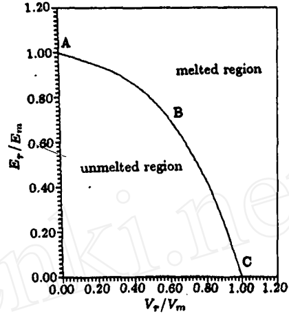
图8 由 V_r/V_m 和 E_r/E_m 确定的熔化区域 Fig.8 Margin curve separating melted and unmelted regions in V_r/V_m \sim E_r/E_m plane
