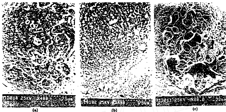
图 1 坑表面熔化特征 Fig.1 Morphology of the crater surface
