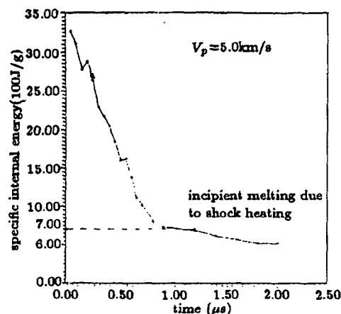
图 2 碰撞点处比内能随时间的变化曲线 Fig.2 Specific internal energy versus time at the impact point
