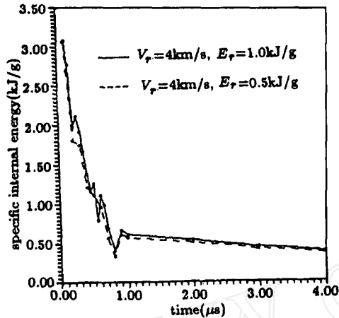
图7 碰撞点处比内能随时间的变化曲线 Fig.7 Variation of specific internal energy of backup material at point of impact with time
