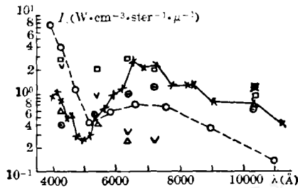
图 4 在状态 A, 各种波长所得实验结果的比较 Fig. 4 Comparison of our results at the state A over various wavelengths with the external results
