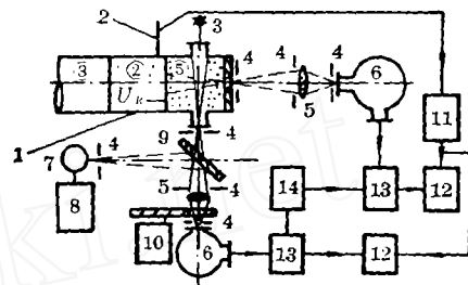
图1 辐射计与激波管匹配示意图 Fig. 1 Diagram showing the match between radiometer and shock tube
