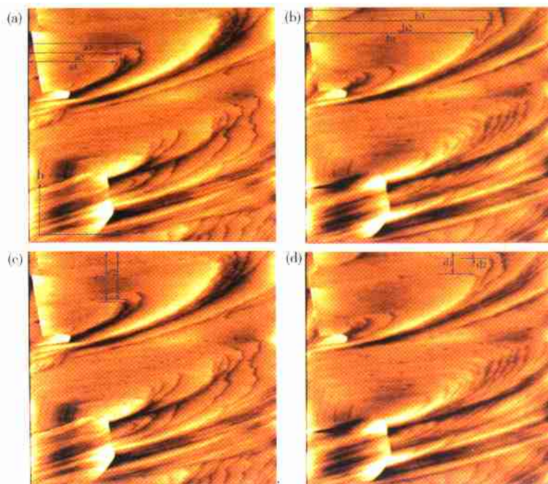
Fig. 1 Series of AFM images taken at 17 min intervals, showing the multi staked 2D islands and expansion of the stack on the {100} surface of EAFP monoclinic crystal at higher supersaturation \sigma = 1.5 , Scan area = 10 \mu\text{m} \times 10 \mu\text{m} , Scan rate = 11 ps.
