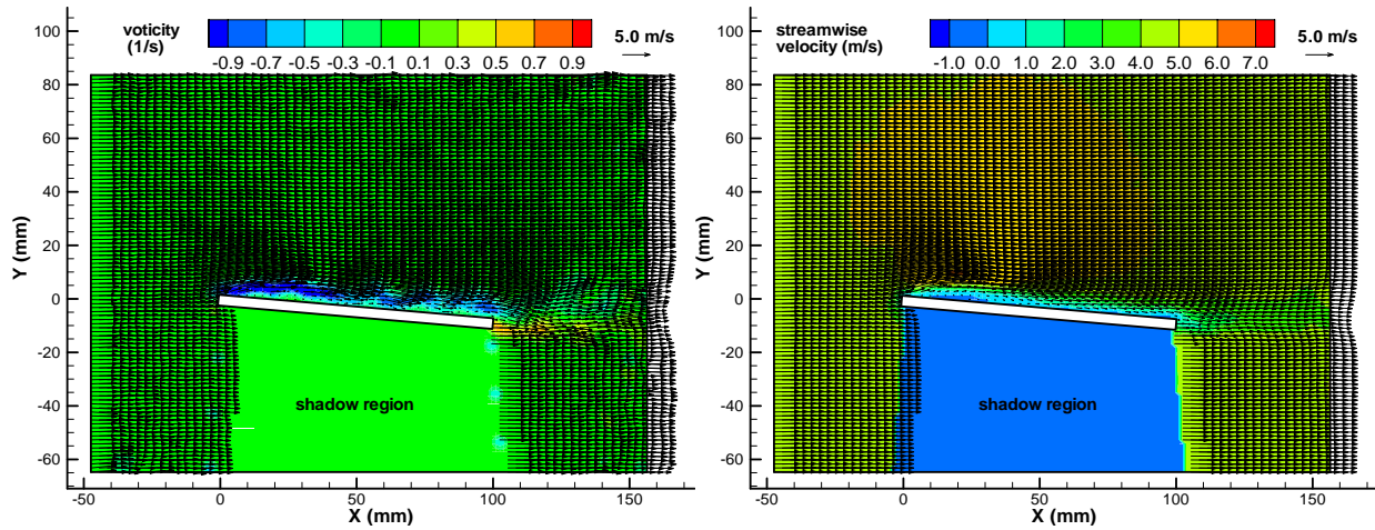
a. Instantaneous velocity field b. Ensemble-averaged velocity field B. flat plate
