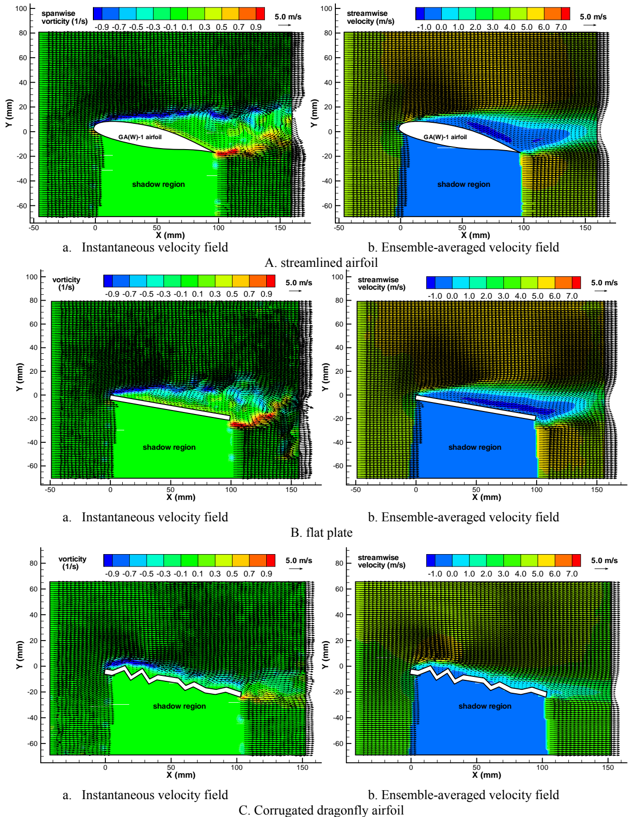
Figure 5 PIV measurement results with AOA=10.0 (Re=34,000)
