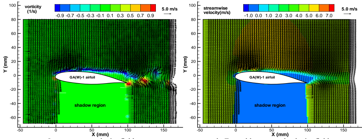
a. Instantaneous velocity field b. Ensemble-averaged velocity field A. streamlined airfoil
