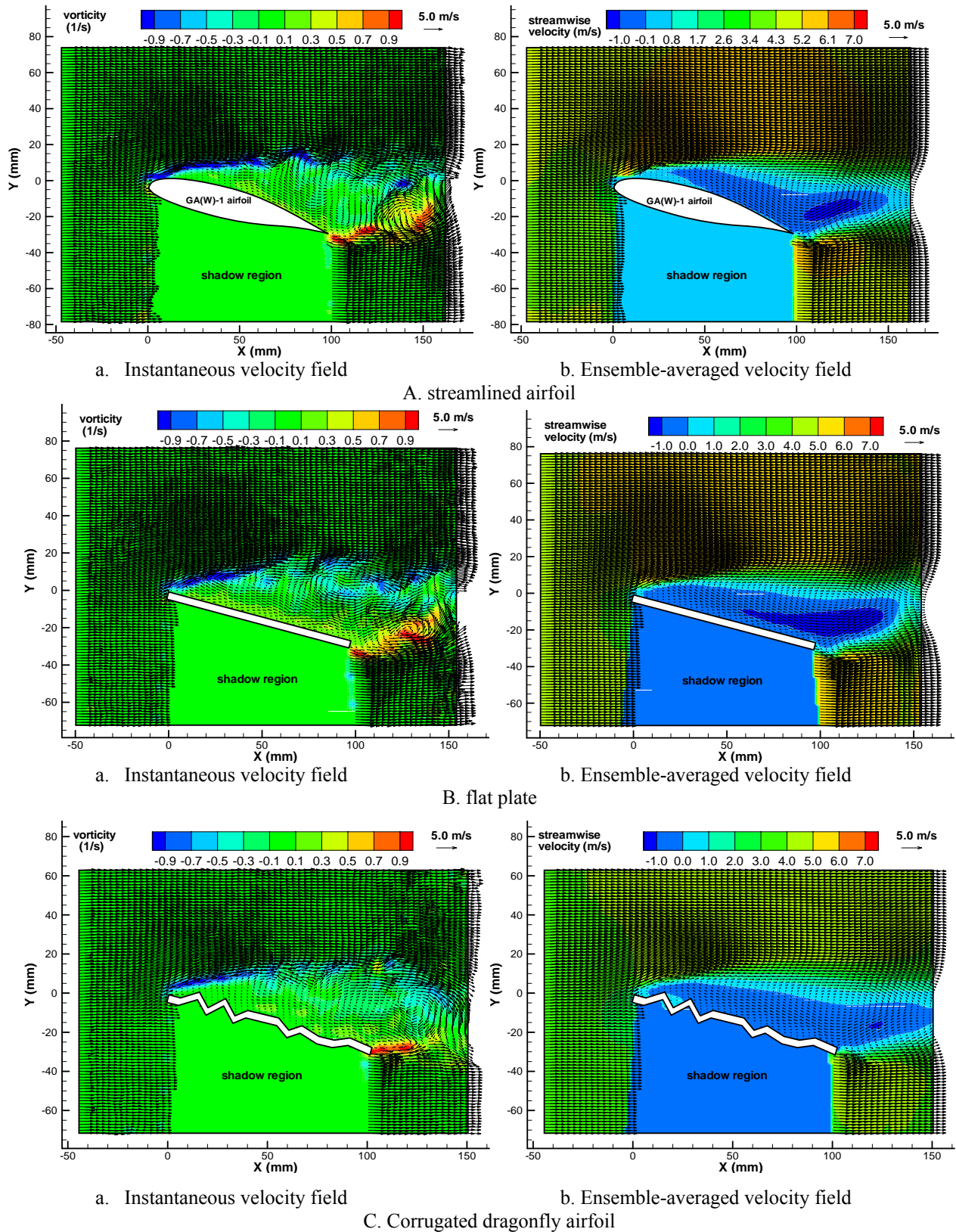
Figure 6 PIV measurement results with AOA=15.0 (Re=34,000)
