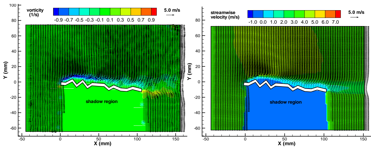
a. Instantaneous velocity field b. Ensemble-averaged velocity field C. Corrugated dragonfly airfoil
