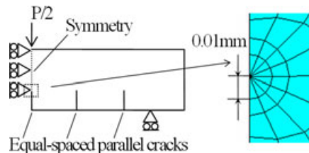
Fig. 3. Finite element model used to determine K_I for the three-point flexure specimen and the crack tip elements.
