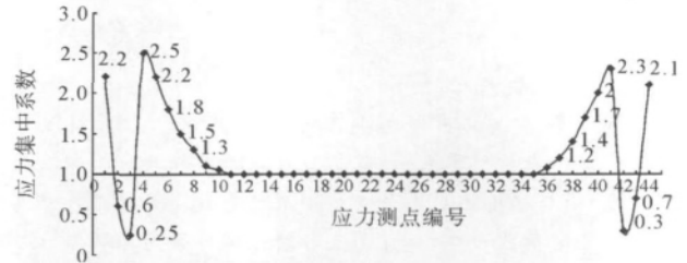
图 7 工作面掘进进风巷后应力测点变化曲线图 Fig. 7 The curves of stress measuring points after driving the face intake airway
