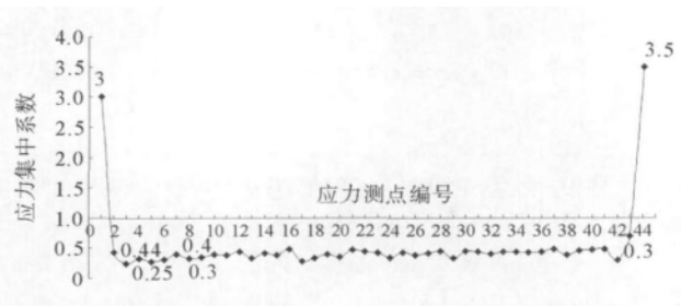
图 8 工作面开采完毕后应力测点变化曲线图 Fig. 8 The curve of stress measuring points after completion of the face mining
