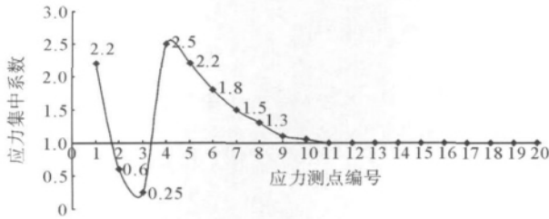
图 6 工作面掘进回风巷后应力测点变化曲线图 Fig. 6 The curves of stress measuring points after driving the face return airway
