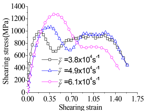
Fig.3 Shearing stress-strain curves
