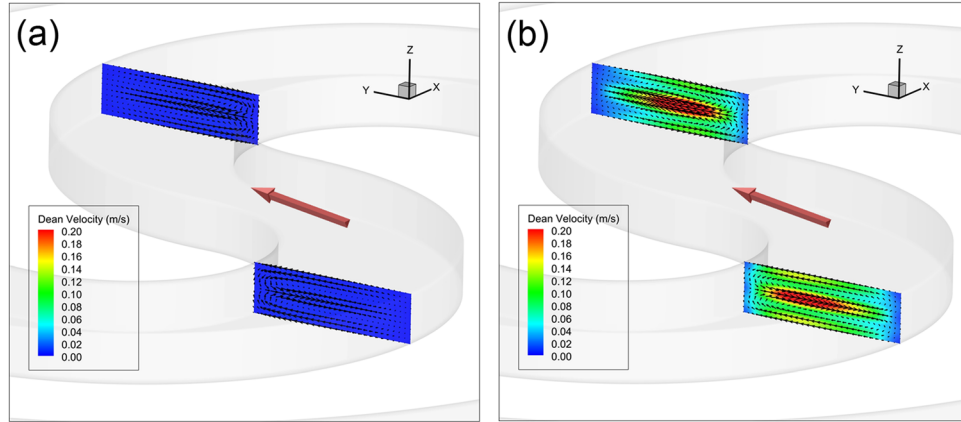
FIG. 2. Comparison of the Dean vortices and their magnitude at (a) 10 ml/h, and (b) 60 ml/h at the S-shape junction. The small arrows represent the velocity vector projected onto the cross-section and color contours represent the magnitude of the Dean flow velocity. The big red arrow indicates the flow direction.
