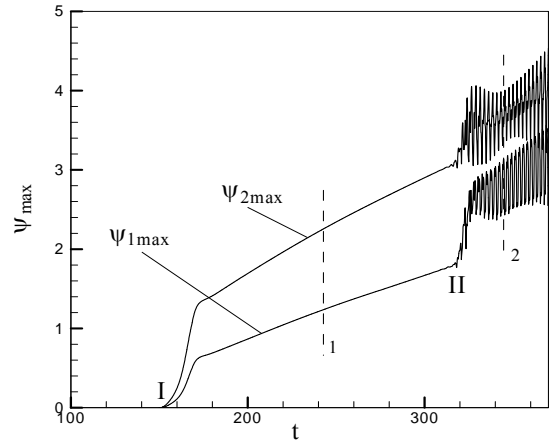
(a) Maximum streamfunction in both layers
