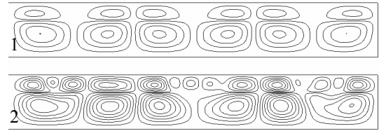
(b) Stream lines
