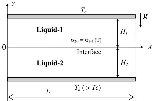
Fig. 1. Schematic diagram of two-layer liquids
