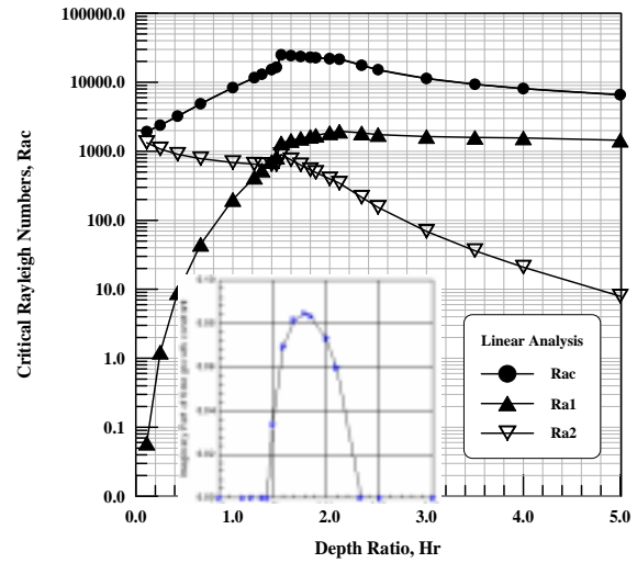
Fig.2. Linear instability analysis: variation of the critical parameters Ra_c , Ra_i , at the onset of R-M-B convection in the system H=6\text{mm} and g=9.8\text{ms}^{-2} for different depth ratios H_r .
