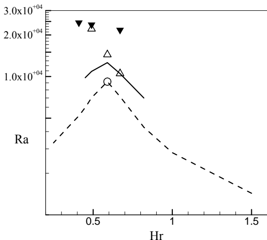
Fig. 5. Comparison of critical Ra for the onset of steady and oscillatory convection in the Silicone oil-water two layer system obtained by different methods: ----- onset of oscillatory convection (linear stability), O onset of steady convection (linear stability), ——— onset of steady convection (2D simulation), \Delta onset of oscillatory convection (2D simulation), and \blacktriangledown onset of oscillatory convection (Degen's expts.).
