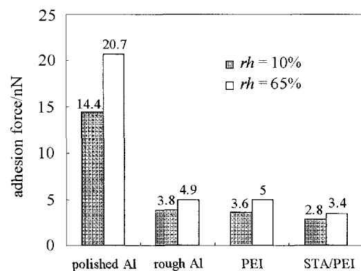
Fig.3 Adhesive forces between an AFM tip and various surfaces at relative humidity of 10% and 65%
