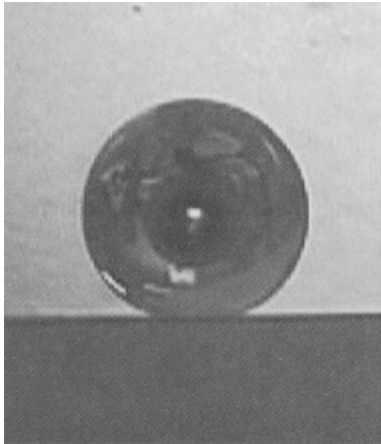
Fig.2 Photo of a water droplet ( \sim 3\mu\text{L} ) on a rough STA monolayer surface with super-hydrophobicity
