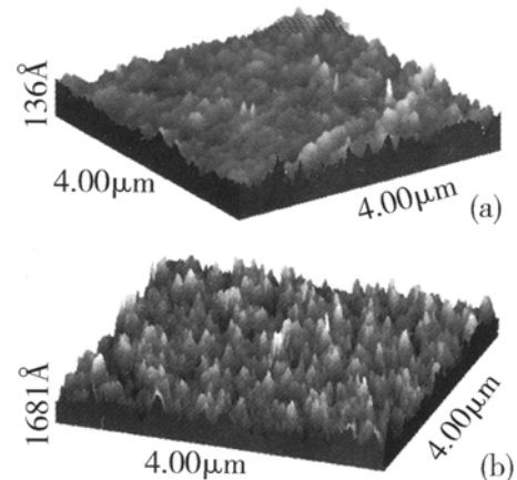
Fig.1 AFM images of polished aluminum wafer (a) and that boiled in water for 5 min (b)
