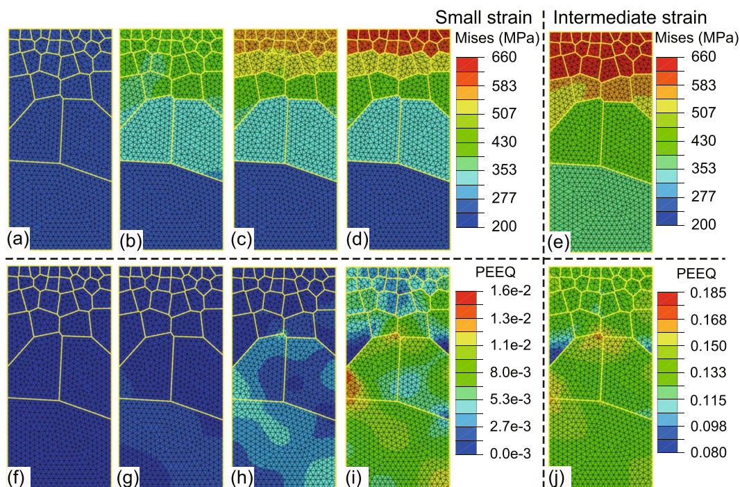
Figure 7. Contours of von Mises stress and equivalent plastic strain from the two-dimensional plane strain sample. (a) to (e) Von Mises stress contours of the P-Gradient structure at points (I) to (V) keyed in Fig. 6, in turn. (f) to (j) The corresponding equivalent plastic strain contours.
