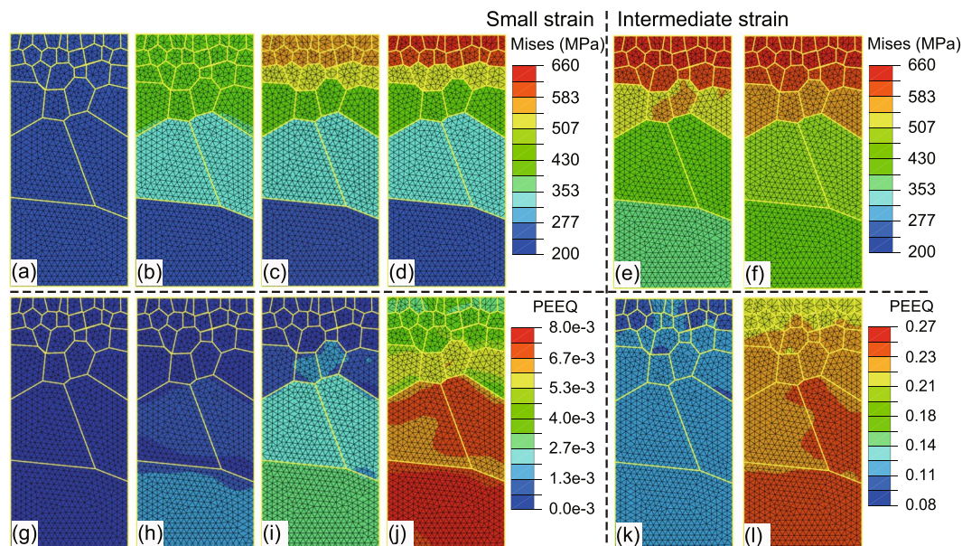
Figure 2. Contours of von Mises stress and equivalent plastic strain of the P-Gradient structure at strains keyed in Fig. 1b. (a) to (f) Von Mises stress contours of the P-Gradient structure at (I) to (VI), in turn. (g) to (l) The corresponding equivalent plastic strain contours of the P-Gradient structure.
