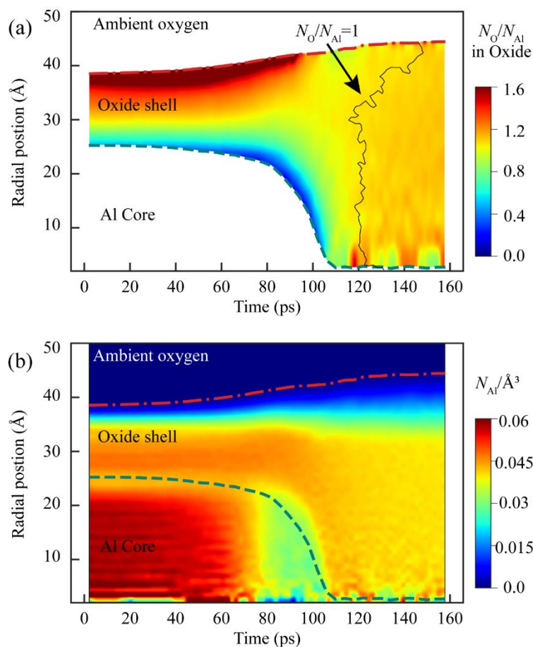
Figure 6 Evolution of ANP structures indicated by atoms distribution contours as well as distribution of O atom number to Al atom number ratio ( N_O/N_{Al} ) in oxide shell (a), and Al atom number density in the whole calculation domain (b). The dash and dash-dot curves are the core-shell interface and ANP surface, respectively.
