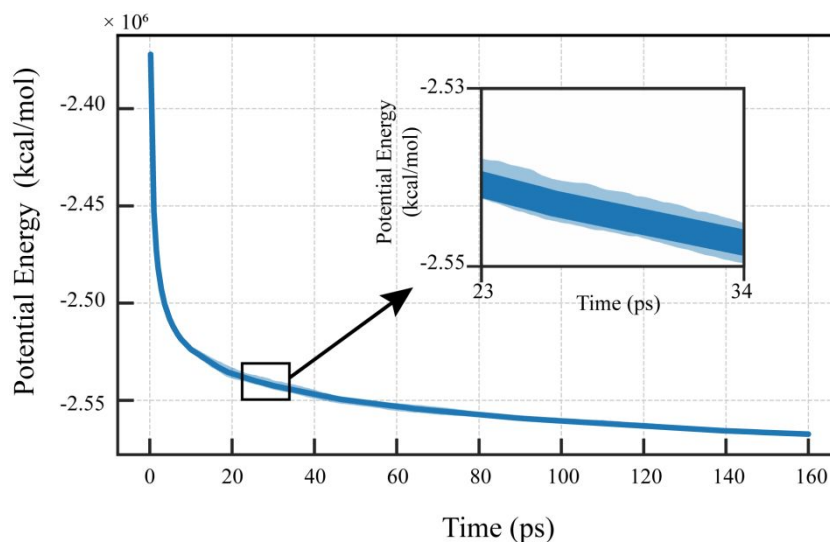
Figure 2 Temporal variation of ANP potential energy during relaxation in NVT ensemble.
