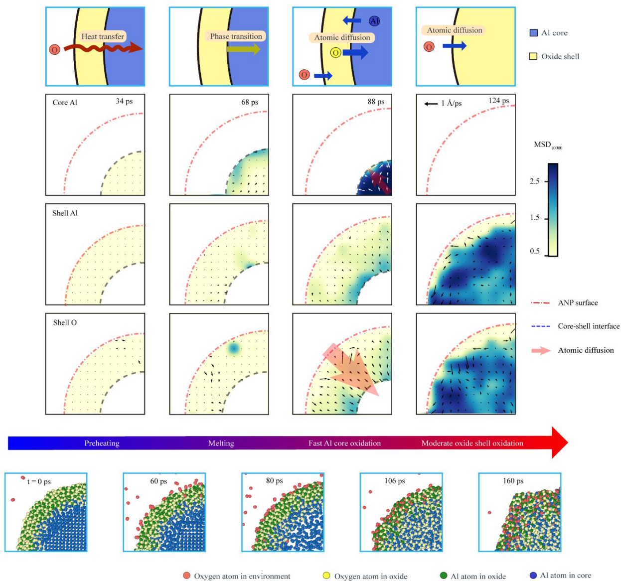
Figure 5 Schematic of heat and mass transfer processes (1 st row), temporal MSD 10000 contour and atomic diffusion vectors of core Al (2 nd row), shell Al (3 rd row) and shell O atoms (4 th row), and snapshots of central cross section of ANP (bottom row).
