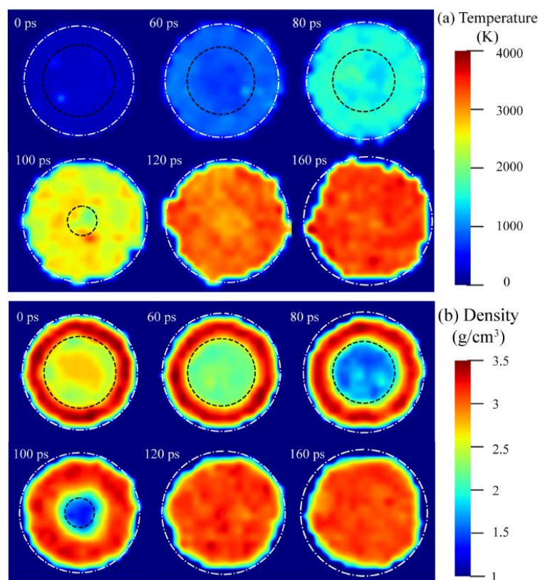
Figure 3 Representative snapshots of the cross sections of temperature (a) and density (b) distributions of ANP. The dash and dash-dot curves represent the core-shell interface and ANP surface, respectively.
