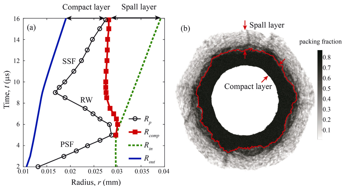
Fig. 6. (a) trajectories of the inner and outer radii of the particle ring in test no.1, R_{in} and R_{out} , the pressure front, R_p , and the boundary delimiting the inner compact layer and outer dilute spall layer, R_{comp} . Here PSF, RW and SSF refer to the primary shock front, the rarefaction wave and the secondary shock front, respectively. (b) Coarse-grained packing fraction field of the explosive dispersed particle ring at t = 17 \mu\text{s} in test no.1. Note that the instantaneous particle ring is composed of an inner compact band with packing fraction \phi \sim 0.84 and an outer spall layer with \phi < 0.6 .
