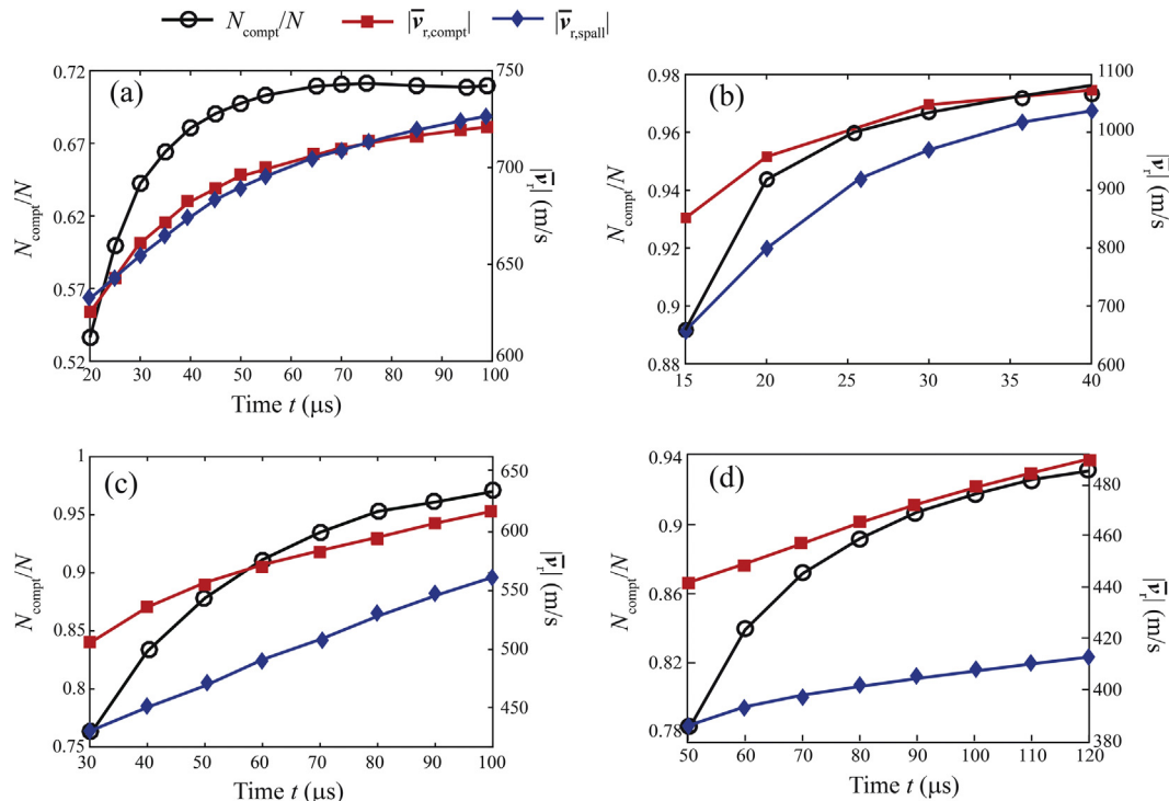
Fig. 14. Variations in average velocities of inner compact bands and spall layers, \bar{v}_{r,\text{compact}} and \bar{v}_{r,\text{spall}} , as well as the fraction of particle number in inner compact band, N_{\text{compact}}/N , for test no. 1 (a), no. 3 (b), no. 5 (c) and no. 6 (d).
