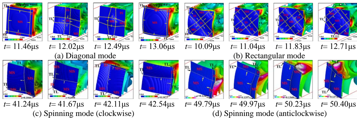
Figure 1. Pressure isosurfaces in about one period when simulating with different initial perturbation and cross-sectional size L , including (a) the diagonal mode (Formula 6 with \kappa=4, L=4 mm), (b) the rectangular mode (Formula 7 with \kappa=2, L=4 mm), (c) the spinning mode (Formula 6 with \kappa=4, L=1 mm, clockwise), and (d) the spinning mode (Formula 7 with \kappa=2, L=1 mm, anticlockwise).
