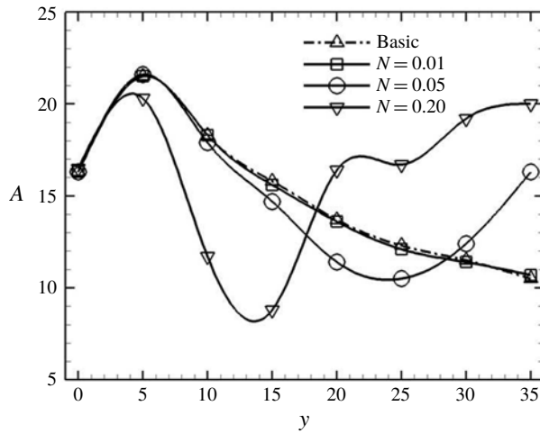
FIGURE 17. Oscillation amplitude with multi-pulse disturbance and N = 0.01, 0.05, 0.20 .
