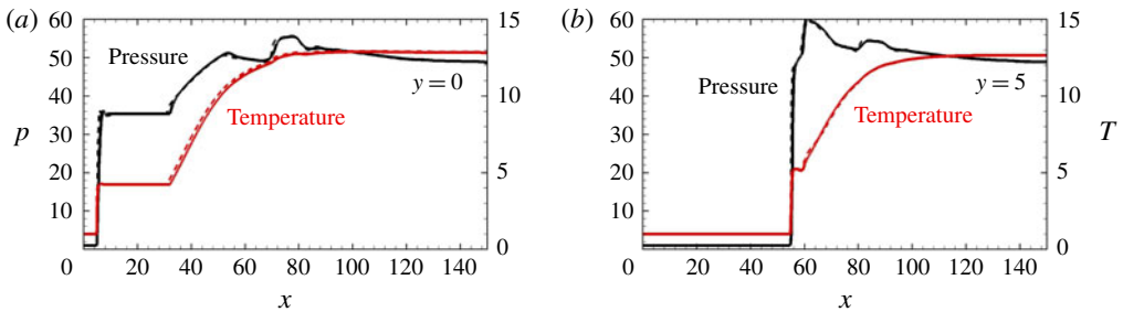
FIGURE 3. (Colour online) Pressure and temperature along the lines y = 0 (a) and 5 (b) with M_0 = 10 , grid 0.10 \times 0.10 (solid) and 0.05 \times 0.05 (dashed).
