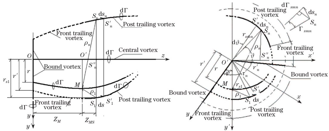
Fig. 6 Induced velocity of post trailing vortex
