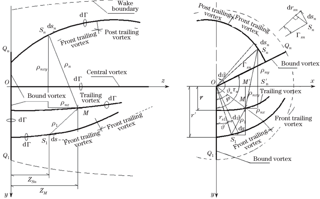
Fig. 5 Induced velocity of front trailing vortex
