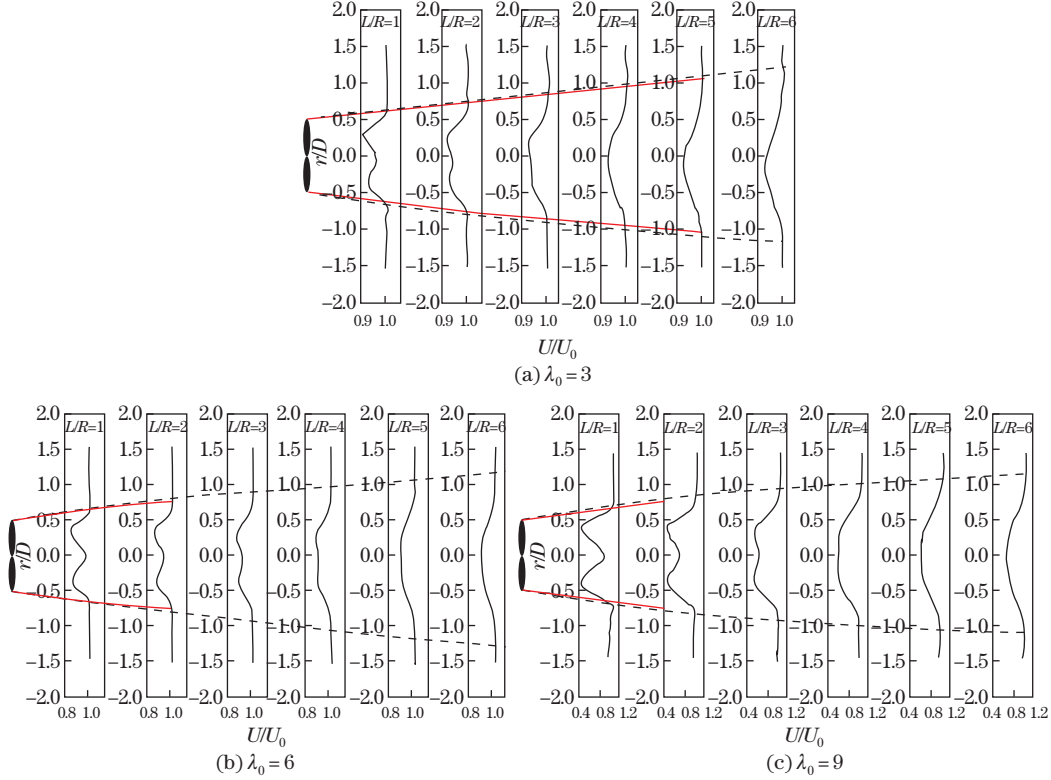
Fig. 8 Spanwise distribution of time-averaged velocity of different tip speed ratios (color online)
