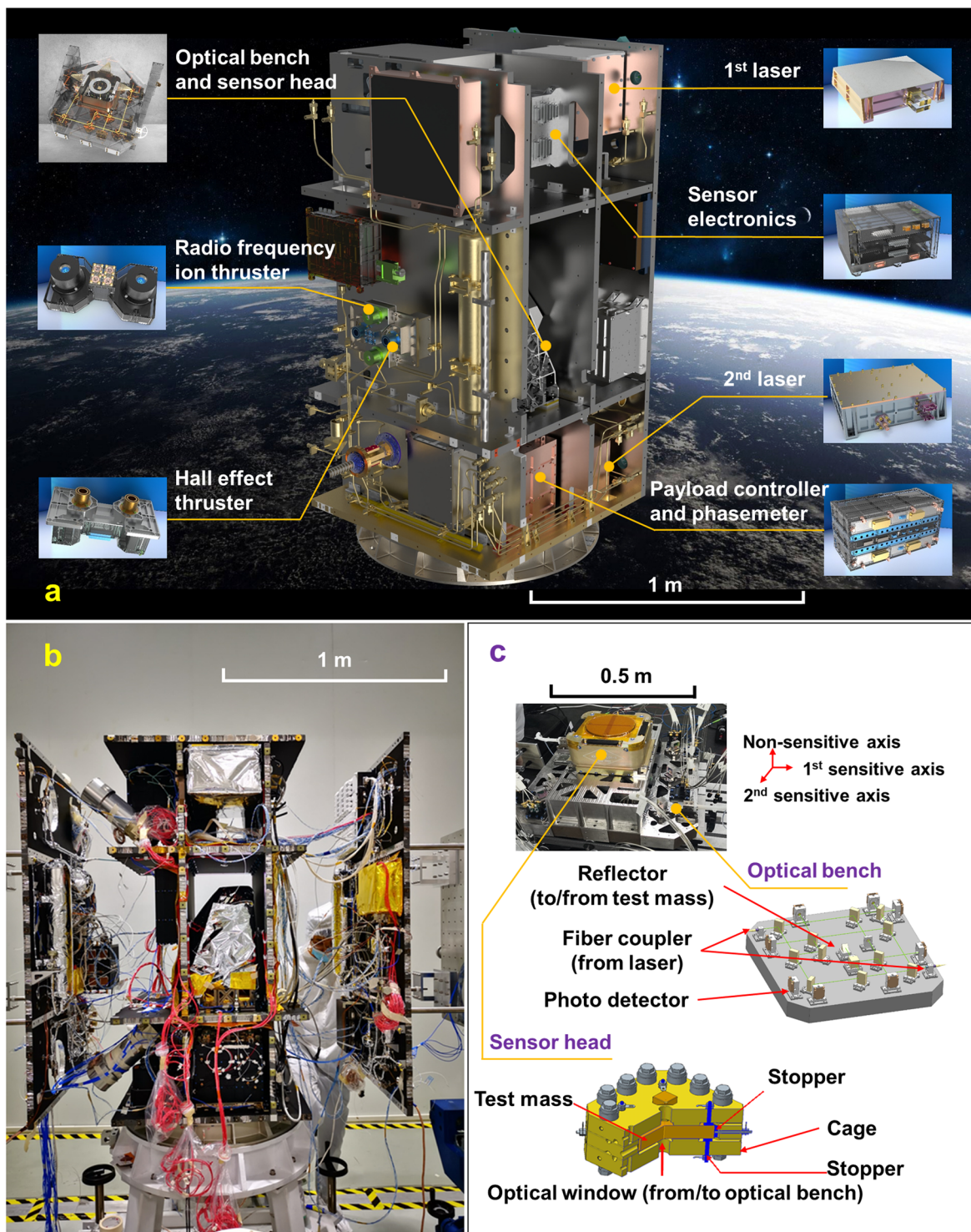
Fig. 1 Anatomy of Taiji-1 and its payloads. a The distribution of the payloads in Taiji-1. The optical bench and the sensor head are integrated in order to ensure the laser beam to get accurate access to the test mass. The difference between the nominal geometric center of the test mass and the mass center of the satellite is smaller than 0.15 mm after the balancing is achieved with a 0.1 mm measurement accuracy. b Taiji-1 satellite before assembling. c The core measurement unit. It contains an optical bench and a sensor head. The plate of the optical bench is made of invar steel, and the mirrors are made of fused silica. The cage of the sensor head is made of the low thermal expansion glass ceramics, and is coated with gold. The test mass is also coated with gold and is made of titanium alloy. The stoppers are used to prevent the test mass from contacting the inner surface of the cage during launch.
