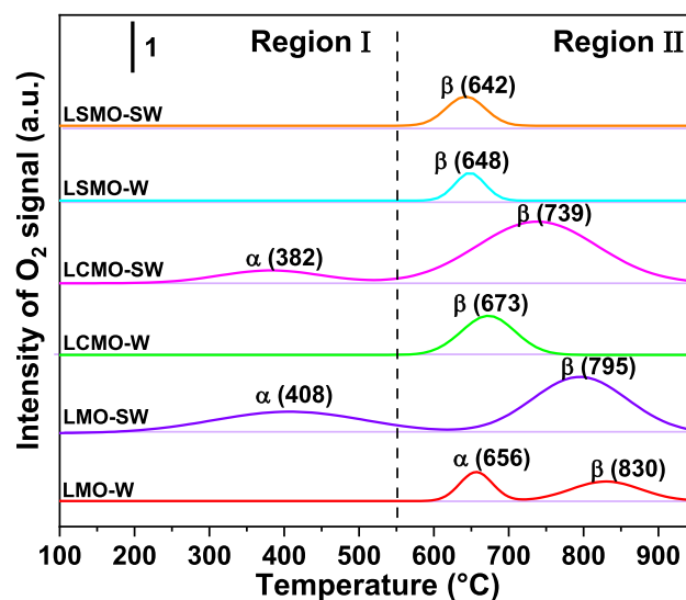
Fig. 4. O 2 -TPD profiles of catalysts.
