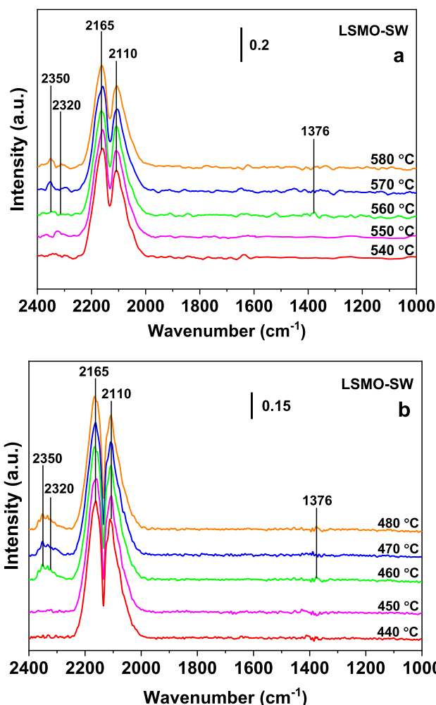
Fig. 11. IR spectra of LSMO-SW catalyst for the CO oxidation at 10 °C intervals under 25% \text{CO}/\text{N}_2 (a) and 25% \text{CO} + 25\% \text{O}_2/\text{N}_2 (b) continuous stream conditions.
