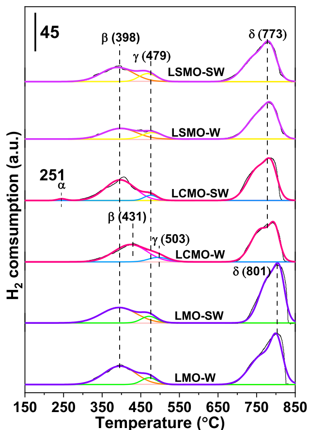
Fig. 3. H 2 -TPR profiles of the catalysts.
