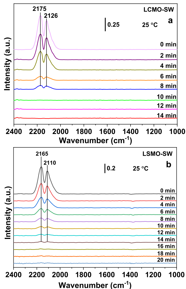
Fig. 9. IR spectra of the LCMO-SW catalyst (a) and LSMO-SW catalyst (b) arising from 25% CO + 25% O 2 /N 2 adsorption/desorption are recorded by 2 min interval under the ambient temperature condition.
