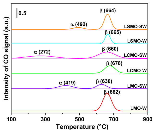
Fig. 5. CO-TPD profiles of catalysts.
