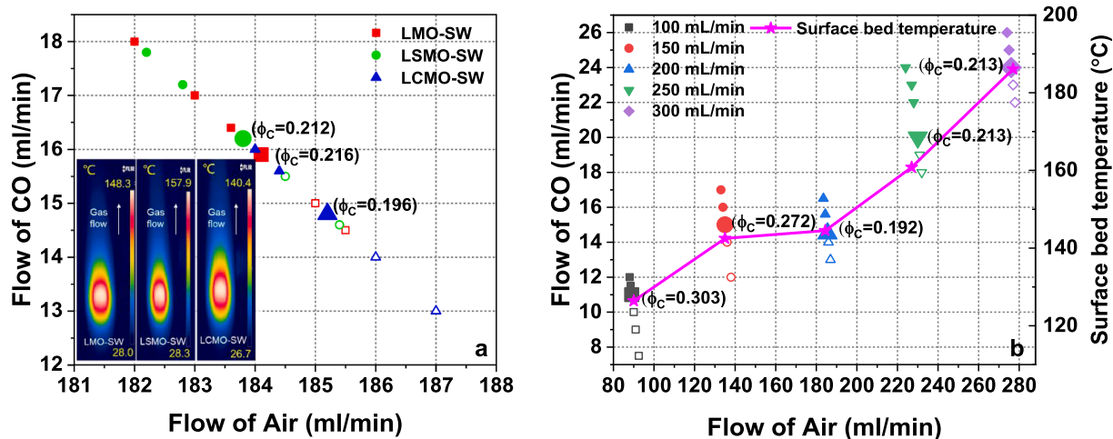
Fig. 8. Lean-combustion limits of CO self-sustained combustion over LMO-SW, LSMO-SW, and LCMO-SW catalysts (a) and over LCMO-SW catalyst in different flow (b).
