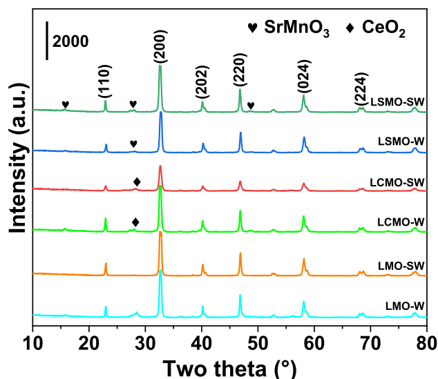
Fig. 1. XRD patterns of the catalysts.
