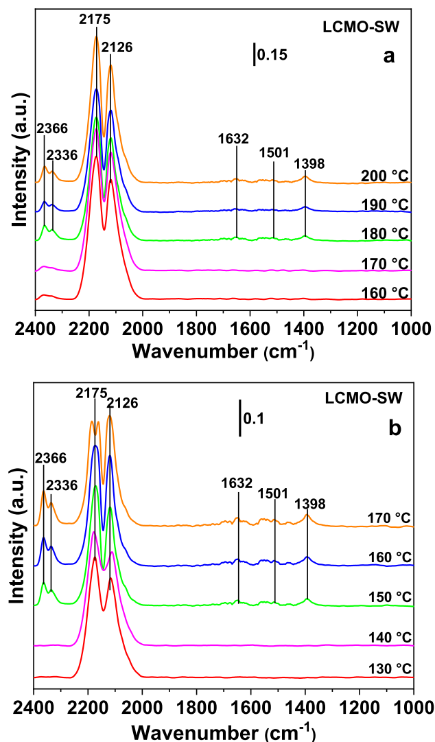
Fig. 10. IR spectra of LCMO-SW catalyst for the CO oxidation at 10 °C intervals under 25% \text{CO}/\text{N}_2 (a) and 25% \text{CO} + 25\% \text{O}_2/\text{N}_2 (b) continuous stream conditions.
