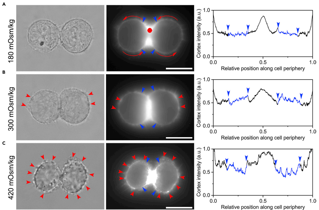
Figure 5. The Laplace pressure changes the cortex structure
