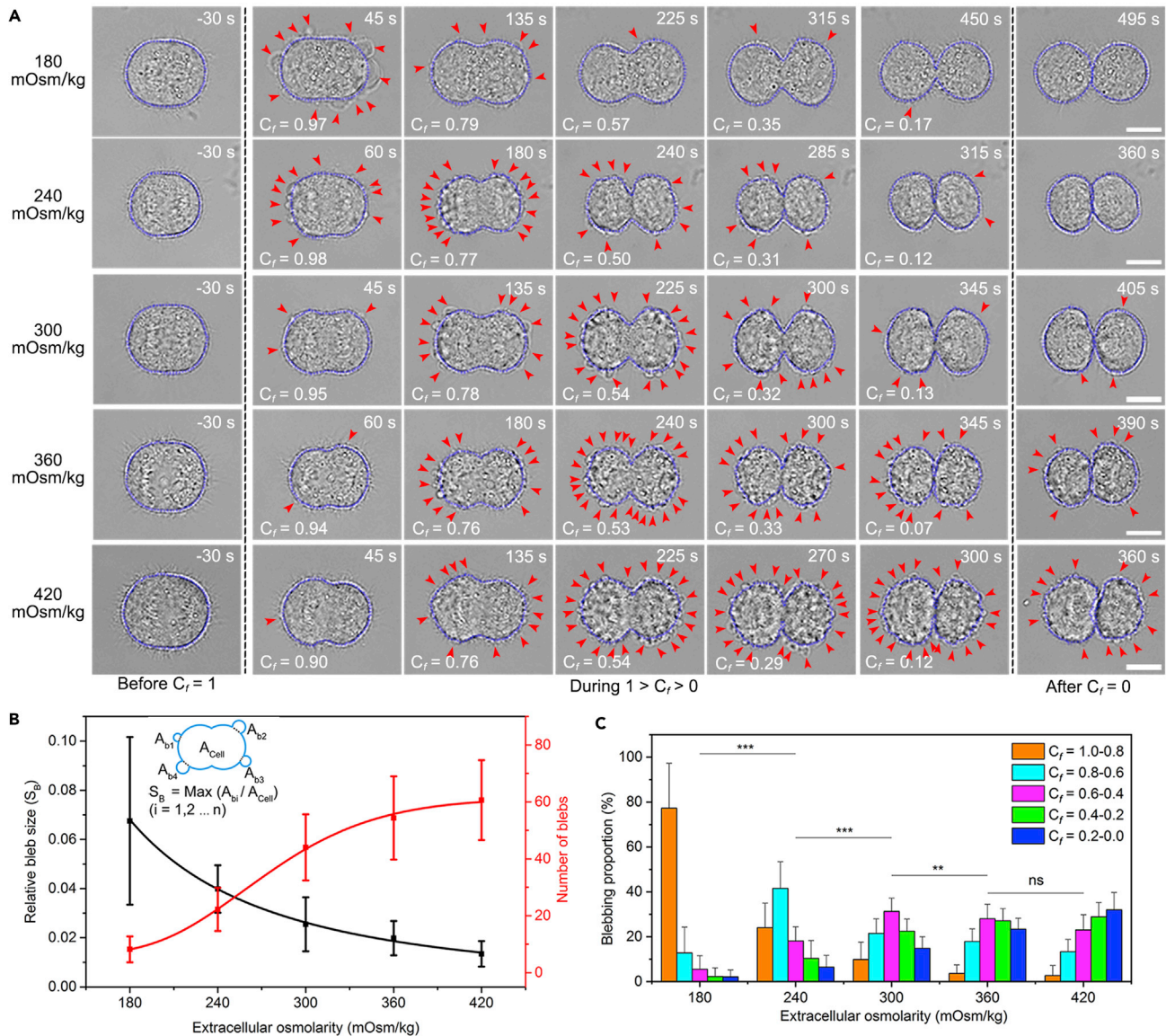
Figure 2. The effect of the Laplace pressure on the blebbing during cytokinesis
