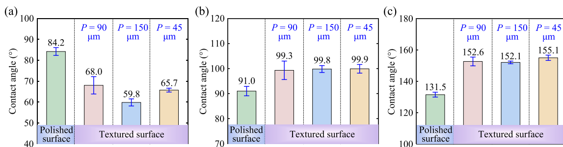
Fig. 4. The CAs of the polished and textured surfaces: (a) without post-processing, (b) after exposing in the air for 100 days, (c) after fluoroalkylsilane modification.
