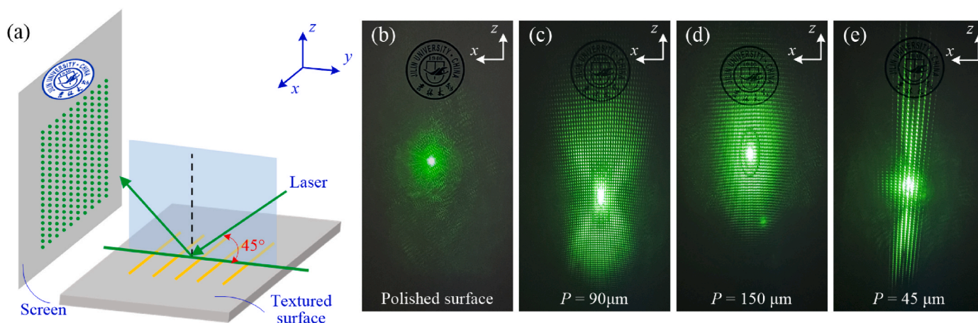
Fig. 3. (a) The schematic of reflection testing. Reflection characteristics of the surfaces under different P : (b) polished surface, (c) P = 90 \mu\text{m} , (d) P = 150 \mu\text{m} and (e) P = 45 \mu\text{m} .
