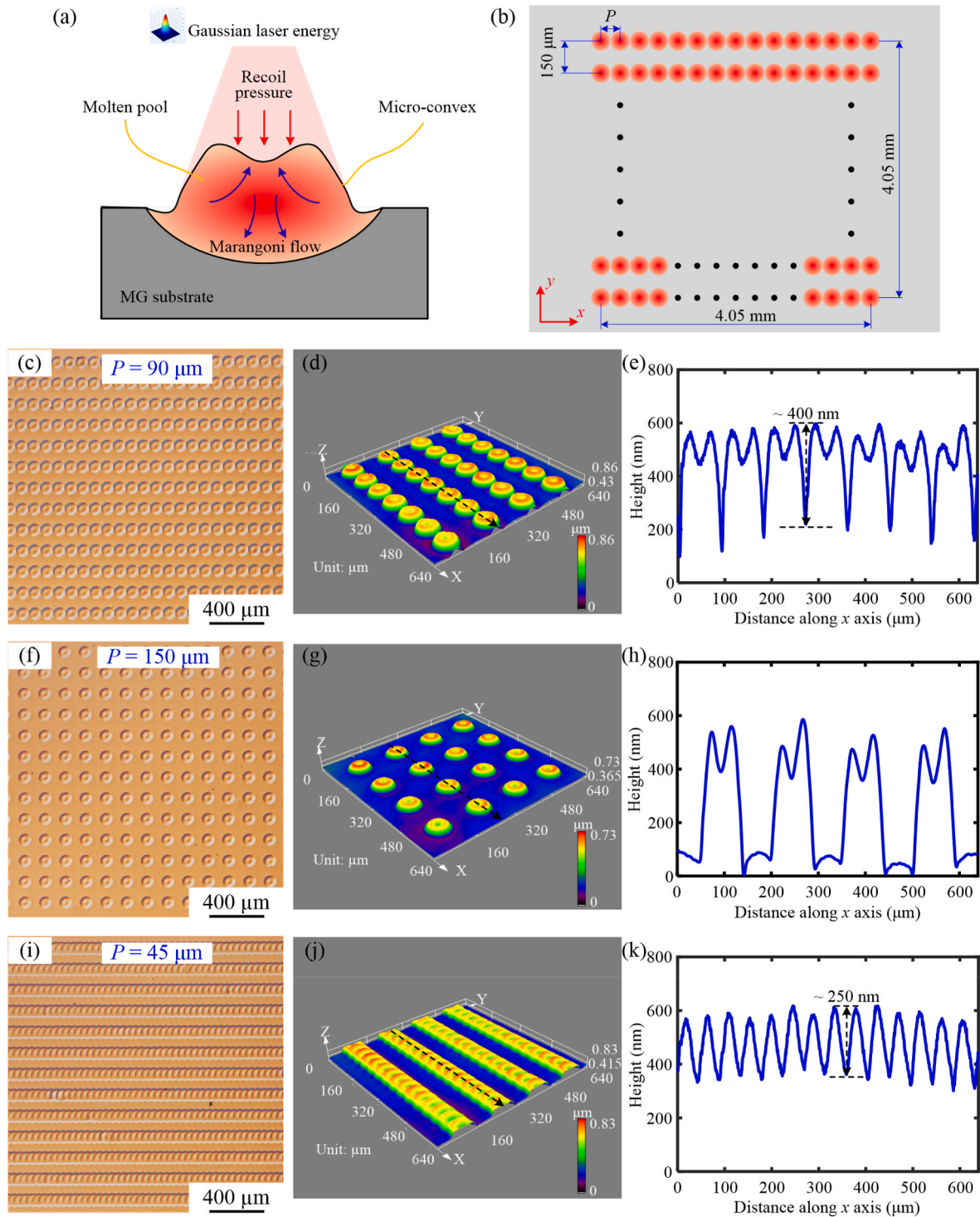
Fig. 1. Schematic diagrams of (a) the formation mechanism of micro-convex structure and (b) the designed micro-convex array structure. Optical images and 3D topographies of the textured surface under different P : (c) and (d) P = 90 \mu\text{m} , (f) and (g) P = 150 \mu\text{m} , (i) and (j) P = 45 \mu\text{m} . (e), (h) and (k) illustrate the cross-section profiles along the mark lines in (d), (g) and (j), respectively.
