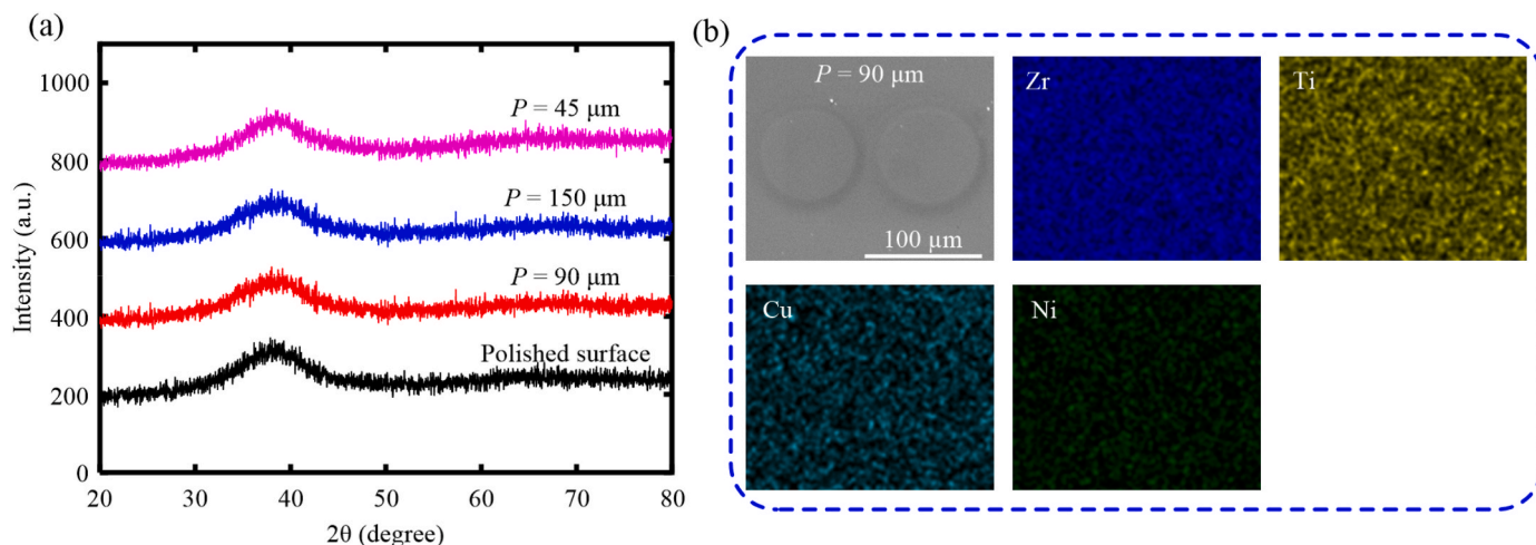
Fig. 2. (a) XRD profiles of the polished and textured surfaces. (b) SEM-EDS analyses of the textured surface under P = 90 \mu\text{m} .
