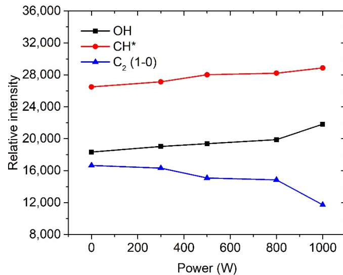
Figure 17. Radiation spectrum of free radicals with power.
