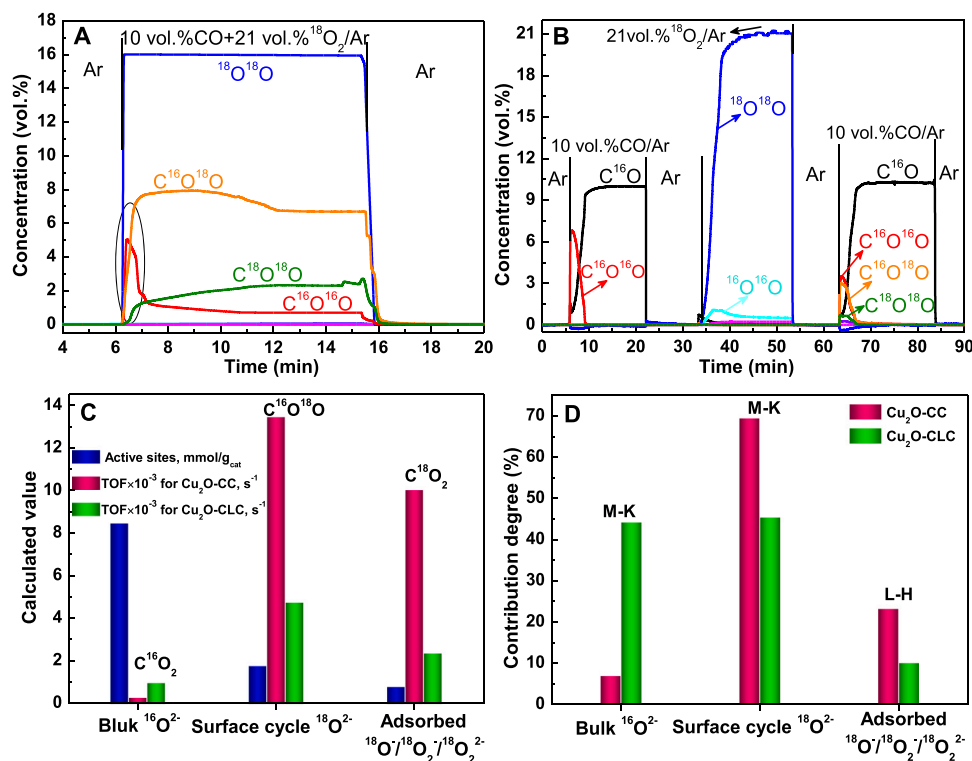
Fig. 9. Isotopic ( ^{18}\text{O}_2 ) exchange experiments over \text{Cu}_2\text{O} for CC (A) and CLC (B) processes at 300\text{ }^\circ\text{C} ; the amount of different active sites and TOF (C), and contribution degree of different mechanisms on active oxygen species (D) for \text{Cu}_2\text{O-CC} and \text{Cu}_2\text{O-CLC} processes.
