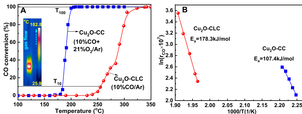
Fig. 2. The catalytic activity and activation energy profiles for \text{Cu}_2\text{O-CC} and \text{Cu}_2\text{O-CLC} processes.
