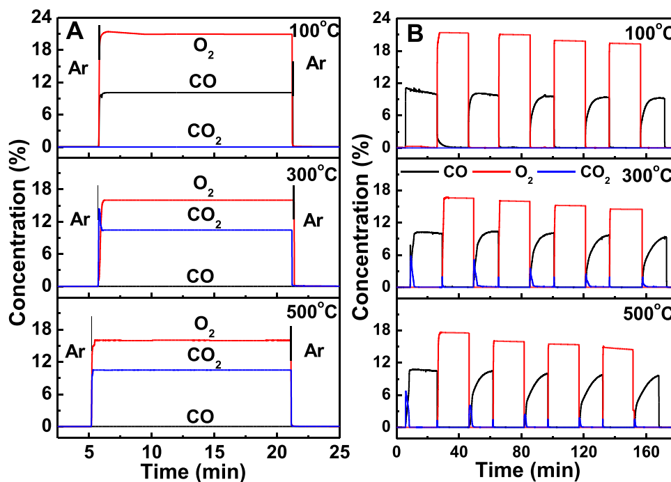
Fig. 3. (A) Catalytic combustion over \text{Cu}_2\text{O-CC} (with 10 vol% CO + 21 vol% \text{O}_2/\text{Ar} ) and (B) chemical looping combustion (with 10 vol% \text{CO}/\text{Ar} and 21 vol% \text{O}_2/\text{Ar} ) over \text{Cu}_2\text{O-CLC} catalyst at different temperatures and time.
