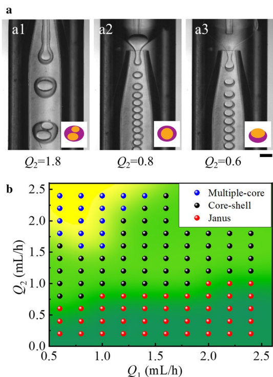
Fig. 2 Generation of microdroplets with different morphologies. The outer and inner diameters of the tip of the collection tube are 425 \mu\text{m} and 250 \mu\text{m} respectively. a Three different generation patterns of compound droplets under different middle volumetric flow rate ( Q_2 ), with the same inner volumetric flow rate, Q_1 = 0.6 mL/h and outer phase volumetric flow rate, Q_3 = 6 mL/h. Subfigures a1 , a2 , a3 correspond to multiple-core, core-shell, and Janus droplets, respectively. The scale bar is 200 \mu\text{m} . See videos for the dynamic process of the generation of the three different compound droplets in Supporting Information (Movies S1–S3). b Regime diagram for droplet types as a function of Q_1 and Q_2 , where Q_3 is fixed at 6 mL/h
