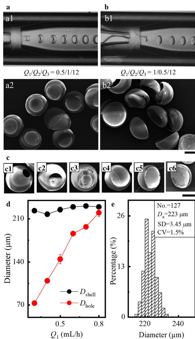
Fig. 7 Controlling the hole size of microparticles. a, b Generations of hole-shell microparticles under Q_1+Q_2=1.5 mL/h and Q_3=12 mL/h, but different Q_1 and Q_2 . a1 and b1 are experimental snapshots and a2 and b2 are SEM images corresponding to a1 and b1 . c Series of SEM images showing that shapes of microparticles change from hole-shell to shallow-bowl-like as the Q_1 increases under Q_1+Q_2=1 mL/h and Q_3=9 mL/h. d Variations of shell diameters and hole diameters corresponding to c . e Distribution of the shell diameters for the microparticles generated under Q_1=0.3 mL/h, Q_2=0.7 mL/h and Q_3=9 mL/h. The average diameter ( D_a ) of 127 shells is 223 \mu\text{m} , with a standard deviation (SD) of 3.45 \mu\text{m} . The coefficient of variation (CV) of the shell diameters is 1.5%. The scale bars are 100 \mu\text{m}
