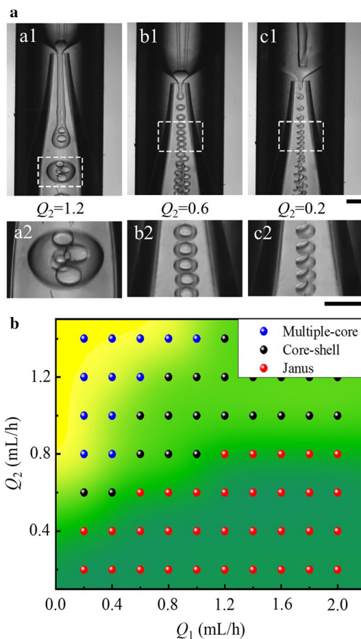
Fig. 3 Generation of microdroplets with different morphologies in a device that has a smaller tip of the collection tube. The outer and inner diameters of the tip of the collection tube are 275 \mu\text{m} and 170 \mu\text{m} , respectively. a Three different generation patterns of compound droplets under different middle volumetric flow rate ( Q_2 ), with the same inner volumetric flow rate, Q_1 = 0.4 mL/h and outer phase volumetric flow rate, Q_3 = 3 mL/h. Subfigures a2 , b2 , c2 correspond to for multiple-core, core-shell, and Janus droplets, respectively. Both scale bars are 200 \mu\text{m} . b Regime diagram for droplet types as a function of Q_1 and Q_2 , where Q_3 is fixed at 3 mL/h
