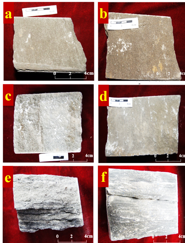
Figure 1. Pictures of the evaluated core samples. (a,b) Show sandstone samples with high oil saturation. (c,d) Indicate sandstone samples with medium oil saturation. (e,f) Display sandstone samples with low oil saturation.
