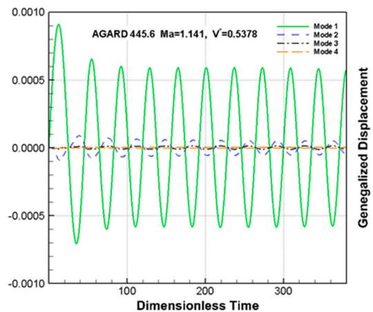
(f) Generalized displacements for Ma = 1.141 and V^* = 0.5378
