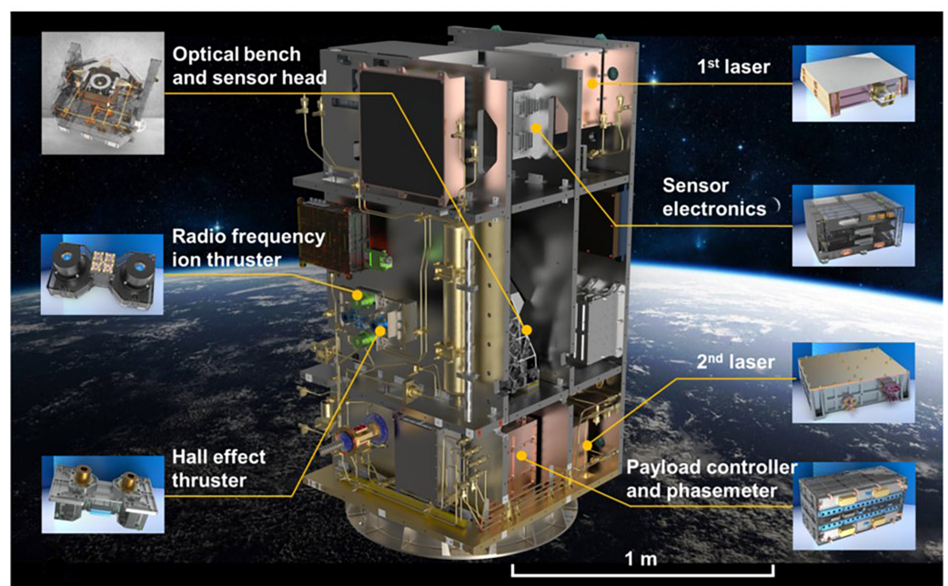
Figure 2. The layout of the payloads of Taiji-1.
