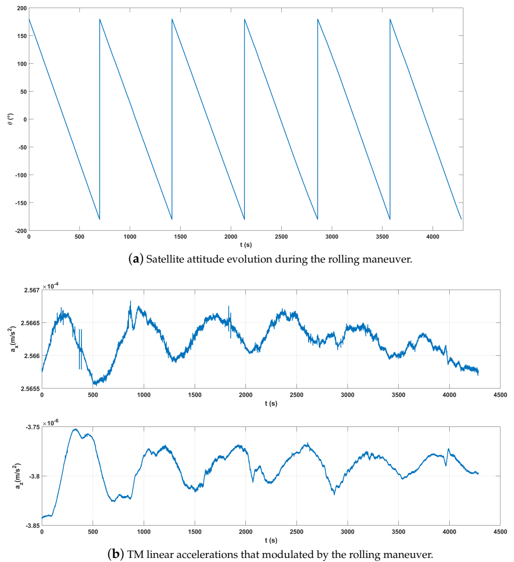
Figure 16. (a) Attitude evolution of the satellite along y-axis during the rolling maneuver. (b) The TM linear accelerations along the x- and z-axes during the rolling maneuver.
