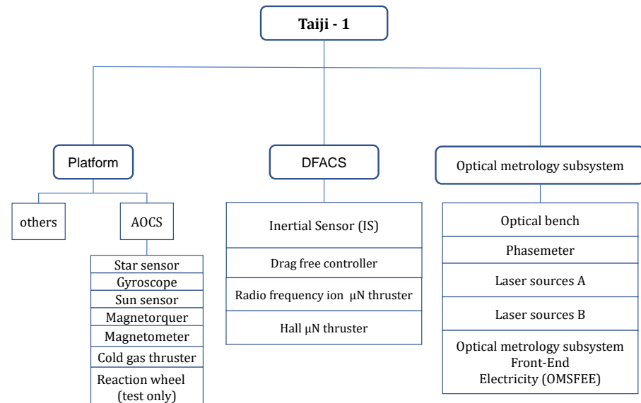
Figure 1. Block diagram for the architecture of Taiji-1.
