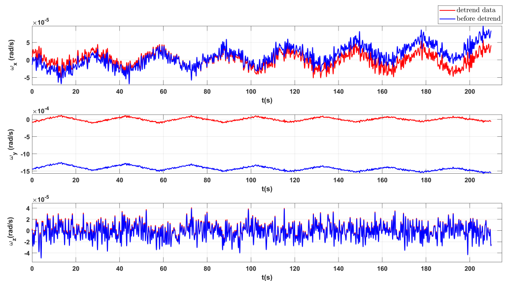
Figure 6. The angular velocity of the satellite measured by star tracker. The blue lines denote the data before detrending and the red lines denote the data after detrending.
