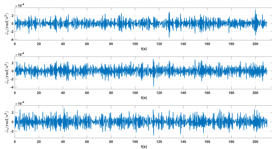
(b) Satellite angular accelerations by star trackers before filtering.
