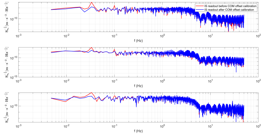
Figure 15. Comparisons of the ASD curves of the TM linear accelerations before (red lines) and after (blue lines) the COM corrections.
