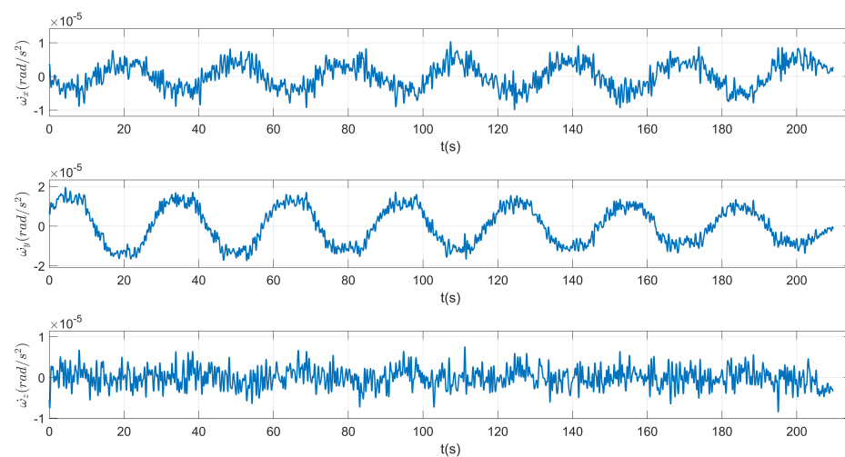
(c) Satellite angular accelerations by star trackers after filtering.
