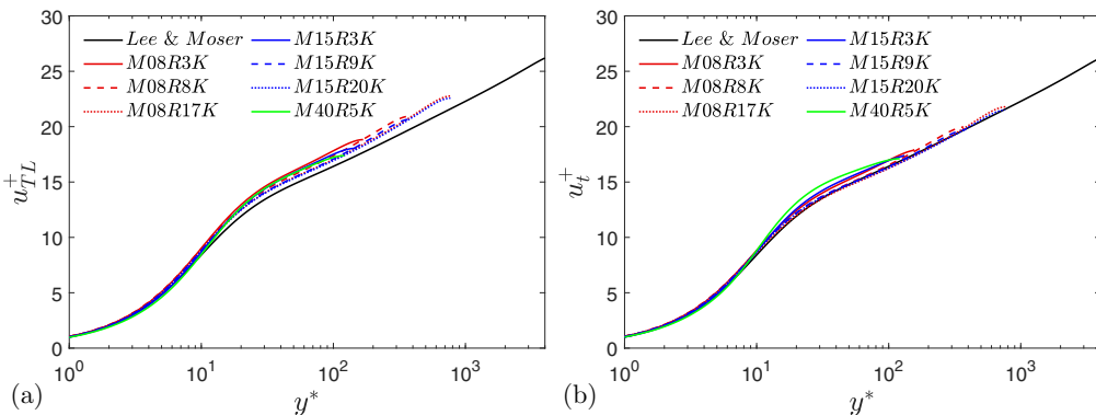
FIG. 22. Mean streamwise velocity profiles transformed by (a) the Trettel-Larsson transformation [28] and (b) the total-stress-based transformation [29]. All the DNS cases in Table I are examined. The black solid line denotes the reference and is taken from the incompressible channel flow with \text{Re}_{\tau} \approx 5200 in Ref. [70].
